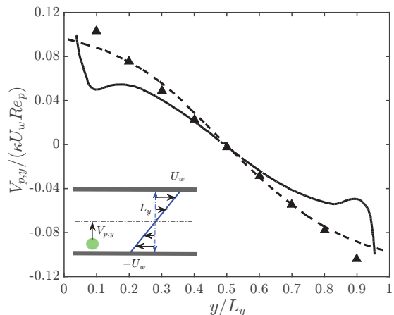
FIG. 3. Quasi-steady wall-normal velocity of a single particle as a function of the particle distance to the wall in laminar pCf. The lines are theoretical predictions from Vasseur and Cox [39] (dashed line) and Ho and Leal [38] (solid line); \blacktriangle present simulation with \kappa = d/L_y = 1/32 , Re_p = 2.4 \times 10^{-4} .
