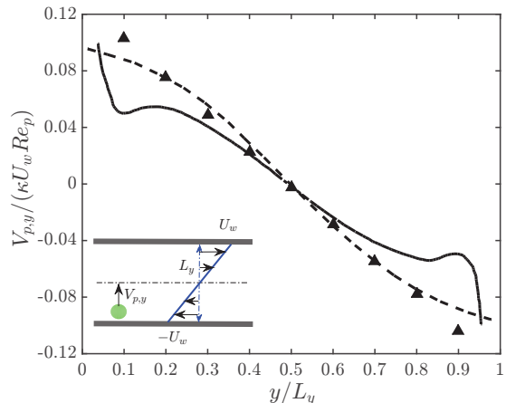
FIG. 3. Quasi-steady wall-normal velocity of a single particle as a function of the particle distance to the wall in laminar pCf. The lines are theoretical predictions from Vasseur and Cox [39] (dashed line) and Ho and Leal [38] (solid line); \blacktriangle present simulation with \kappa = d/L_y = 1/32 , Re_p = 2.4 \times 10^{-4} .
