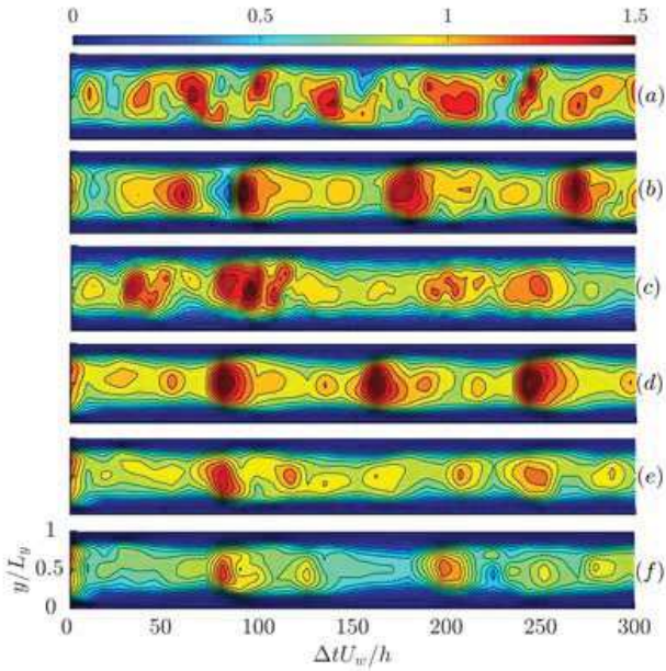
FIG. 25. Evolution in time of shear Reynolds stress \overline{u'^+v'^+}(y, t) averaged over the homogeneous directions. (a) and (b) are for single phase flow at Re_b=500 and 380 respectively. (c) to (f) correspond to two-phase flow simulations at Re_b = 500 , \Phi = 10\% and different particle size and inertia. In (c), L_y/d = 10 and \rho_p/\rho_f = 1 . In (d), L_y/d = 20 and bubbles are used. In (e), L_y/d = 20 and \rho_p/\rho_f = 2 . Finally in (f): L_y/d = 20 and \rho_p/\rho_f = 5 .
