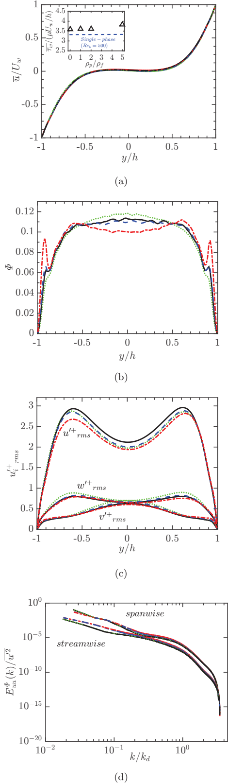
FIG. 18. Effect of inertia on the turbulent flow statistics. Mean profiles of (a) streamwise flow velocity, (b) concentration and (c) r.m.s. of velocity fluctuations. (d) contains TKE spectrum as a function of streamwise and spanwise wavenumbers ( L_y/d_{20} = 20 and k_d = 2\pi/d_{20} ). The line style is the same as in Fig. 16.
