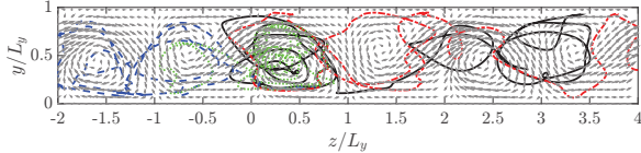
FIG. 16. Effect of particle inertia on the trajectory of a single particle in turbulent pCf at Re_b = 500 . \cdots bubble; \text{---} \rho_p/\rho_f = 1.0 ; \text{---} \rho_p/\rho_f = 2.0 ; \text{---} \rho_p/\rho_f = 5.0 .
