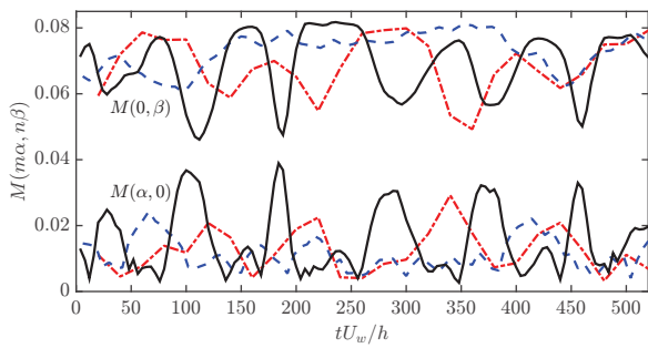
FIG. 22. Modal decomposition: M(0, \beta) and M(\alpha, 0) . The solid lines are for single-phase flow with effective Reynolds number Re_s = 380 ; The two-phase flow simulations are obtained for neutrally-buoyant particles using \Phi = 10\% and Re_b = 500 and --- L_y/d = 10 ; --- L_y/d = 20 .
