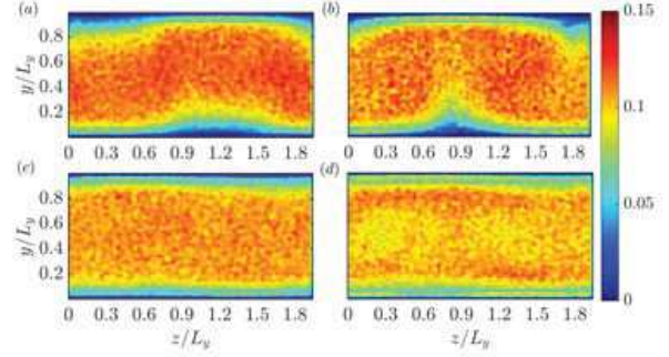
FIG. 17. Contour of particle concentration in the transverse y - z plane averaged over \sim 400 time units. (a): Bubble; (b): \rho_p/\rho_f = 1.0 ; (c): \rho_p/\rho_f = 2.0 ; (d): \rho_p/\rho_f = 5.0 .
