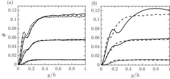
FIG. 9. Concentration profiles for different Reynolds numbers, particle sizes and bulk concentrations. From bottom to top \Phi : 1, 5 and 10%. In (a) L_y/d = 20 and — Re_b = 500 ; --- Re_b = 750 ; - - - Re_b = 1000 . In (b) Re_b = 500 and — L_y/d = 10 ; - - - L_y/d = 20 .
