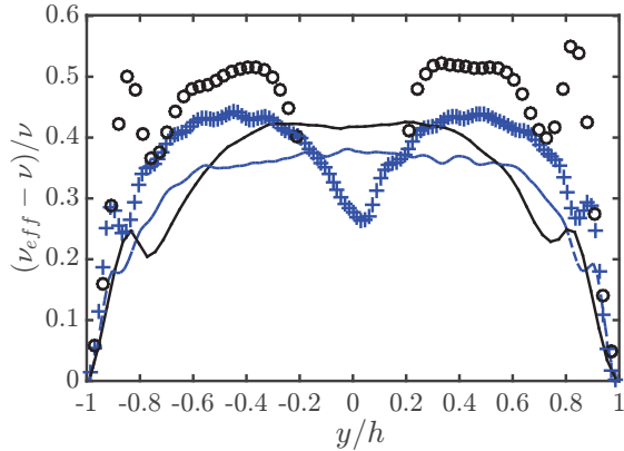
FIG. 14. Profiles of relative mixture viscosity across the Couette gap for Re_b = 500 , \Phi = 10\% and two particle sizes L_y/d = 10, 20 . Eilers fit ([1 + 1.25\Phi/(1 - \Phi/0.63)]^2 - 1.0) based on the local concentration ( \Phi(y/h) ) for two particle sizes: — L_y/d = 10 ; - - - L_y/d = 20 ; Eq. (14) based on the local shear stress: \circ L_y/d = 10 ; + L_y/d = 20 .
