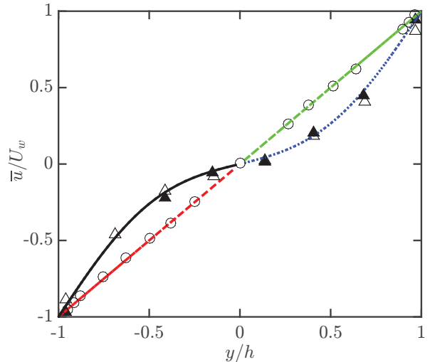
FIG. 6. Streamwise velocity profile in wall-normal direction starting from fluid at rest. Lines correspond to our simulations: \cdots Re_b = 365, \eta = 0.1 ; \text{—} Re_b = 650, \eta = 0.1 ; \text{---} Re_b = 300, \eta = 1.0 ; \text{-.-.-} Re_b = 345, \eta = 1.0 , where \eta is the dimensionless time scaled with h^2/\nu . Symbols stand for experimental or direct numerical simulation results. \Delta Tillmark and Alfredsson [48], Re_b = 365, \eta = 0.1 ; \blacktriangle Tillmark and Alfredsson [48], Re_b = 650, \eta = 0.1 ; \circ Reichardt [49], Re_b = 300 when flow is fully-developed; \bullet Tillmark and Alfredsson [48], Re_b = 345 when flow is fully-developed.
