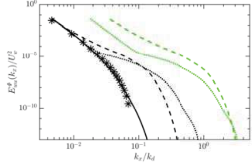
FIG. 12. TKE spectrum as a function of wavenumber in streamwise direction. Single phase of Re_b = 500 scaled by k_d = 2\pi/\delta_\nu : * stretched mesh; — regular mesh for L_y/d = 20 . Two-phase flow with \Phi = 10\% and Re_b = 500 for two particle sizes: --- L_y/d = 10 and ..... L_y/d = 20 , scaled by k_d = 2\pi/\delta_\nu ; - - - L_y/d = 10 , scaled by k_d = 2\pi/d_{10} ; ..... L_y/d = 20 , scaled by k_d = 2\pi/d_{20} . d_{10} and d_{20} correspond to particle diameter and \delta_\nu is the viscous lengthscale based on single-phase flow.
