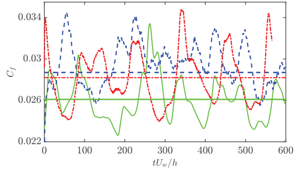
FIG. 8. Temporal evolution of the wall friction coefficient ( C_f , averaged on both walls) at Re_b = 500 . — single-phase flow; - - - L_y/d = 10 , \Phi = 10\% ; ···· L_y/d = 20 , \Phi = 10\% . Straight lines stand for temporal averages.
