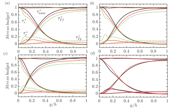
FIG. 15. Profiles of the shear stress budget components for different Reynolds numbers, particle sizes and bulk concentrations. Plots in (a) to (c) compare single-phase flow results (solid line) to two-phase flow simulations (dashed lines) at \Phi = 5\% and \Phi = 10\% . In (d) the shear stress components are compared at \Phi = 5\% — L_y/d = 10 and - - - L_y/d = 20 .
