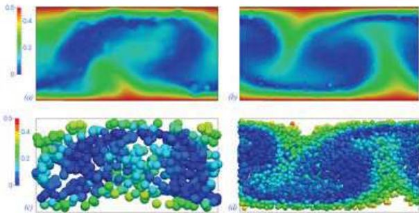
FIG. 10. Top panels: contours of the magnitude of the streamwise flow velocity in the middle cross section. Bottom panels: particle positions projected on the plane ( y, z ), colored according to local magnitude of streamwise velocity. Comparison between L_y/d = 10 (Left) and 20 (right) for Re_b = 500 and \Phi = 5\% .
