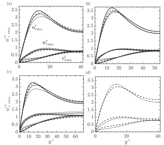
FIG. 11. Profiles of velocity r.m.s. for different Reynolds numbers, particle sizes and bulk concentrations. (a) Re_b = 500 , L_y/d = 20 ; (b) Re_b = 750 , L_y/d = 20 ; (c) Re_b = 1000 , L_y/d = 20 ; (d) Re_b = 500 , \Phi = 5\% . Half of the domain is shown because of mid-plane symmetry. From (a) to (c): — \Phi = 0 ; - - - \Phi = 1\% ; - - - \Phi = 5\% ; ..... \Phi = 10\% . In (d): - - - L_y/d = 10 ; ..... L_y/d = 20 .
