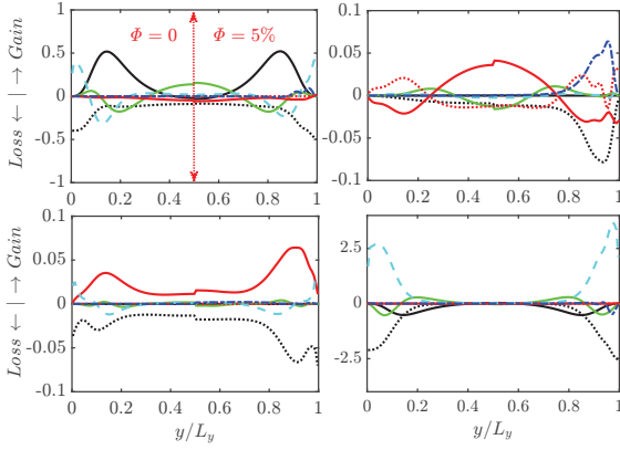
FIG. C1. Contributions to the budget of (a): \overline{u'u'} , (b): \overline{v'v'} , (c): \overline{w'w'} and (d): \overline{u'u} in the case of Re_b = 500 and L_y/d = 20 . Comparison between single phase and \phi = 5\% suspension flow. Because of symmetry of profiles, in each figure the left part correspond to single phase flow and the right part stands for two-phase flows. — Production; .....Dissipation; — Turbulent transport; — Pressure strain; - - - Pressure diffusion; - - - Viscous diffusion; - - - Dipole feedback.
