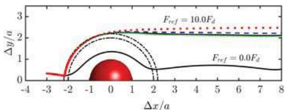
FIG. 1. Relative trajectory of a particle pair in laminar Couette flow, in the case of neutrally buoyant, inertial particles and bubbles. The red half sphere represents the reference particle. The semicircle of radius 2a is the limit of particle overlapping. The other semicircle indicates the barrier corresponding to R_{ref} = 2.2a where the repulsion force is enabled. The particle Re_p \equiv \gamma a^2/\nu = 1.0 and St \equiv (2Re_p\rho_p)/(9\nu\rho_f) varies between 0.2 and 2. — Neutrally-buoyant particle; - - \rho_p/\rho_f=5 ; • \rho_p/\rho_f=10 ; ••••• bubble.
