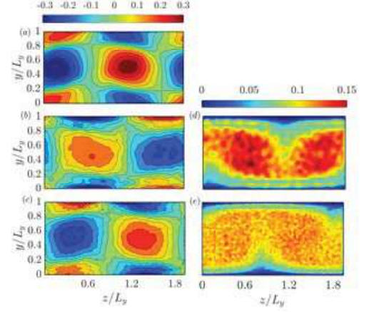
FIG. 19. Streamwise vorticity averaged over \sim 500 time units, comparison between (a) Re_b = 500 single-phase flow and (b), (c) Re_b = 500 , \Phi = 10\% for two particle sizes L_y/d = 10, 20 , respectively. The corresponding contours of concentration projected onto the transverse plane ( yz -plane) is shown in (d) and (e).
