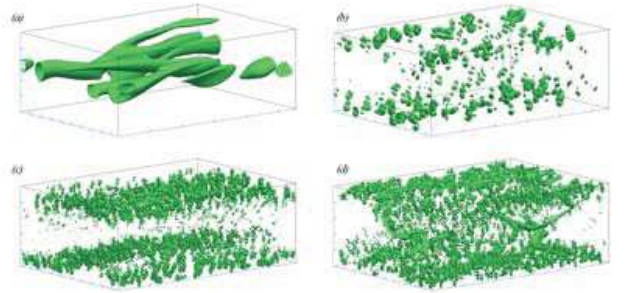
FIG. 13. Vortex identification for single-phase flow and two-phase flows using \lambda_2 criterion. (a): single-phase flow with Re_b = 500 using \lambda_2 = -0.1 ; \Phi = 5\% and \lambda_2 = -1.0 for the followings. (b): L_y/d = 10 and Re_b = 500 ; (c): L_y/d = 20 and Re_b = 500 ; (d): L_y/d = 20 and Re_b = 1000 .
