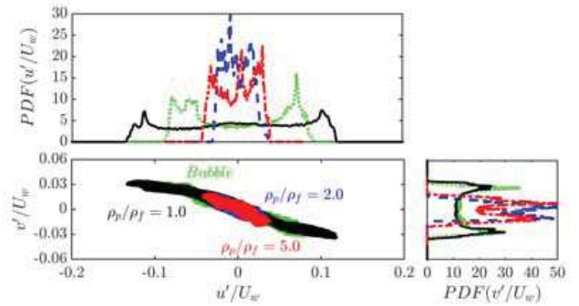
FIG. 21. Effect of particle inertia on the modification of the quadrant analysis of u' and v' and of their probability Density Functions (PDF) in the Couette center plane, for L_y/d = 20, \Phi = 10\% and Re_b = 500 . The line style is the same as Fig. 16.
