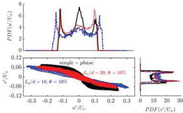
FIG. 20. Modification by the neutrally buoyant particles of the quadrant analysis of u' and v' and of their probability Density Functions (PDF) in the Couette center plane. The single phase plots in solid lines are performed at the effective Reynolds number of the suspension flow ( Re_s = 380 ). Other lines are from two-phase simulations at \Phi = 10\% and Re_b = 500 . --- L_y/d = 10 ; -.-.- L_y/d = 20 .
