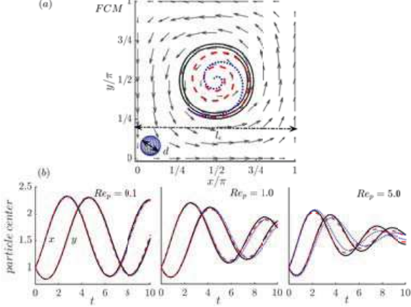
FIG. A1. Trajectory of a bubble ( \rho_p/\rho_f = 1.257 \cdot 10^{-3} ) in a Taylor-Green vortex at different Re_p . (a) trajectory in x - y plane. — Re_p = 0.1 ; - - - Re_p = 1.0 ; ···· Re_p = 5.0 . (b) shows comparison of the FCM results with the numerical solution of Eq. (A1): — Eq. (A1); - - - Eq. (A1) with adding the lift force from Eq. (A3) and Eq. (A2); ···· present simulation.
