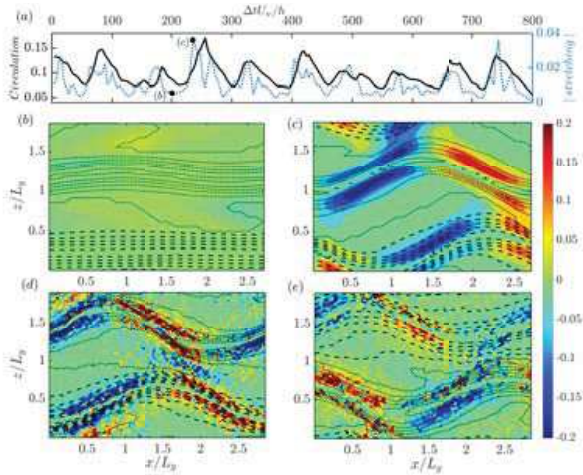
FIG. 24. (a) Profile of — Circulation and - - - - spacial average of absolute value of vorticity stretching ( |\omega_x \partial u / \partial x| within 0.2 < y < 0.4 where LSVs take place as seen in Fig. 19) in single-phase flow and Re_b = 380 , (b-e) Contours of the streamwise velocity fluctuations u'/U_w in the snapshot plane in the center of Couette gap ( y/L_y = 0.5 ), showing the streak structures. The iso-contour interval is 0.07. - - - - stands for u'/U_w < 0 and - - - - stands for u'/U_w > 0 . The color contours indicate the stretching term \omega_x \partial u / \partial x . (a) and (b) are for single-phase flow and Re_b = 380 , with x-independent flow (at the crest of the circulation instant \Delta t U_w / h = 200 ) and for x-dependent flow (at the peak of the circulation \Delta t U_w / h = 235 ) respectively. The crest and peak instants are noted by dots in the panel (a) at the top of this figure. The contours in (c) and (d) are both x-dependent with bubbles and inertial particles ( \rho_p / \rho_f = 5 ) respectively.
