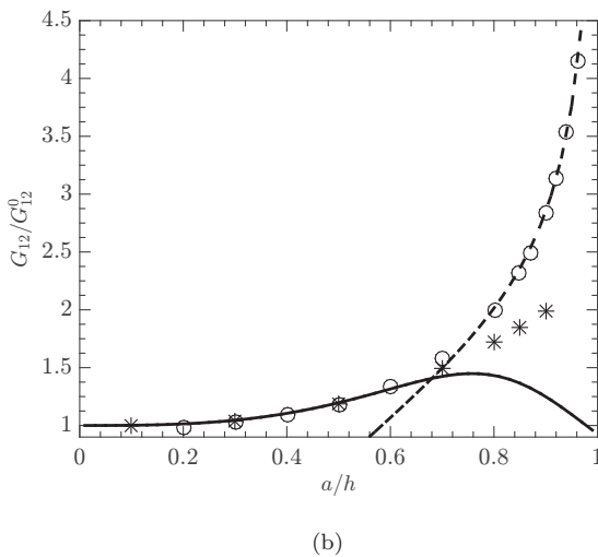
FIG. 2. (a) Rotational velocity and (b) Stresslet of a neutrally-buoyant sphere at the center of laminar pCf as a function of the ratio between the particle radius and half of the gap width a/h . The rotational velocity is scaled by the flow shear rate \gamma , and the stresslet is scaled by its value in unbounded shear flow G_{12}^0 = \frac{10}{3} \pi \mu a^3 \gamma . The stars * are obtained using FCM simulations at Re_p = 0.01 , and circles \circ are from simulations of Sangani et al. [34] in Stokes flow. The lines are from asymptotic limits written in [34]: — a/h \ll 1 ; -- -0 \ll a/h < 1 ;
