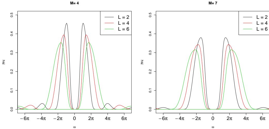
Figure 2. Plot of |\widehat{\psi}_H(\lambda)| for different values of M and L , with Q_{L,M} mid-phase factorisations of R_{L,M} in Theorem 2.2.
