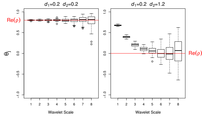
Figure 4. Boxplot of the empirical correlations of the wavelet coefficients \{\theta_j, j \geq 0\} for analytic wavelets in terms of the scales. In red, the real part of the theoretical value of \rho of the ARFIMA model.
