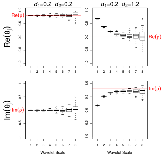
Figure 4. Boxplot of the empirical correlations of the wavelet coefficients \{\theta_j, j \geq 0\} for analytic wavelets in terms of the scales. In red, the real part of the theoretical value of \rho of the ARFIMA model.
