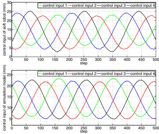
Fig. 5. Control inputs of soft robot and simulation mode using the closed-loop controller
