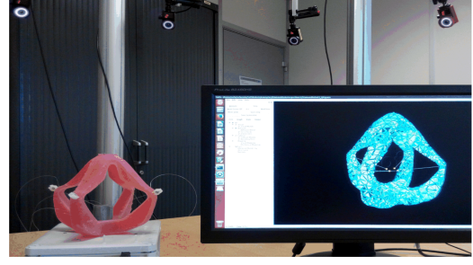
Fig. 3. Experimental setup for trajectory tracking of soft robot. The robot has four soft legs and is actuated by cables. The simulation model serves as a simulation-based predictor. The 3D position of the end effector can be obtained by the position perception system.
