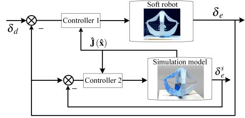
Fig. 2. The implementation of closed-loop controller. Controller 1 and Controller 2 are the closed-loop controllers for the soft robot and the simulation model, respectively. The two controllers can be designed independently.
