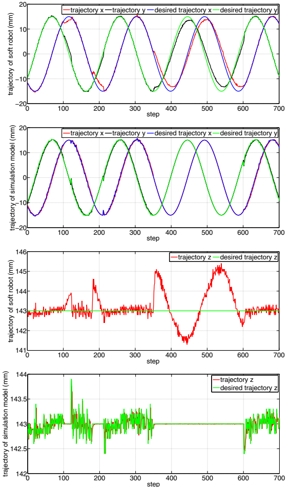
Fig. 6. End effector trajectories of soft robot and simulation model using the switched control strategy.
