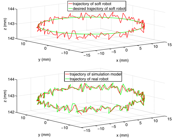
Fig. 4. 3-D trajectories of real robot and simulation model using the closed-loop controller.
