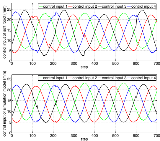
Fig. 7. Tracking control inputs of soft robot and simulation model using the switched control strategy.
