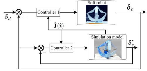
Fig. 2. The implementation of closed-loop controller. Controller 1 and Controller 2 are the closed-loop controllers for the soft robot and the simulation model, respectively. The two controllers can be designed independently.
