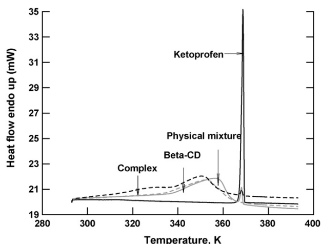
Fig. 5. Differential scanning calorimetry thermograms of ketoprofen, \beta -cyclodextrin, physical mixture and complex.
