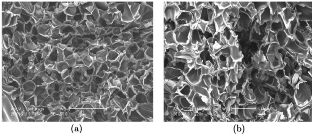
Figure 5 SEM pictures of samples processed at T = 110^{\circ}\text{C} , (a) N = 40 rpm and 0.126% of \text{CO}_2 , (b) N = 80 rpm and 0.068% of \text{CO}_2 (Experiments 1 and 3).
