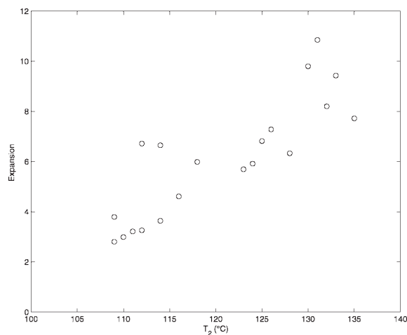
Figure 6 Expansion according to the melt temperature.
