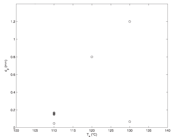
Figure 7 Cell size according to the die temperature.
