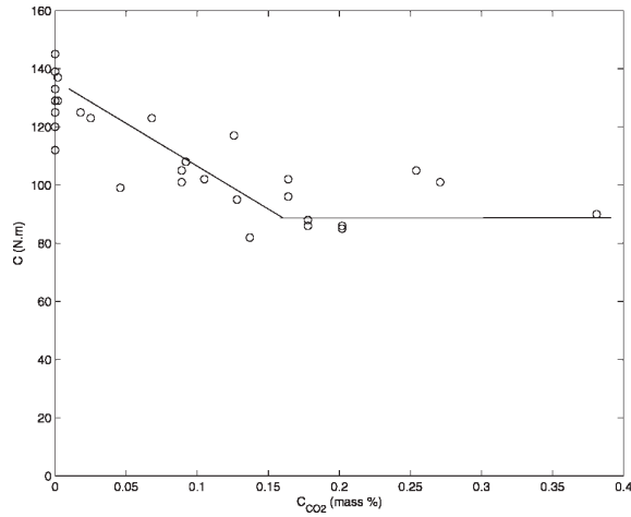
Figure 3 Torque according to the CO 2 concentration.
