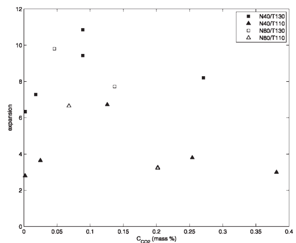
Figure 10 Expansion according to the \text{CO}_2 concentration.
