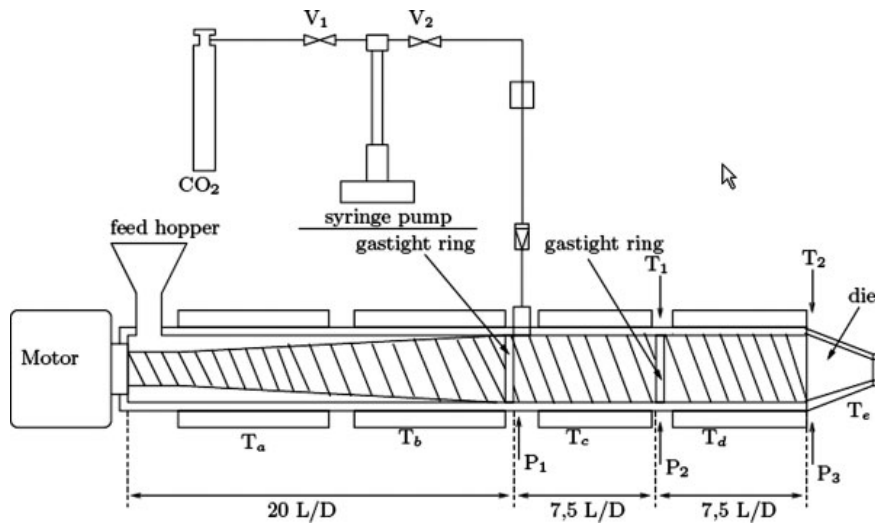
Figure 2 Experimental system.
