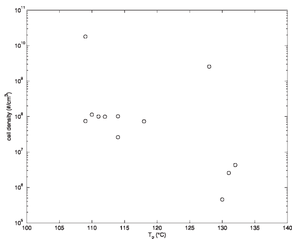
Figure 9 Cell density according to the melt temperature.
