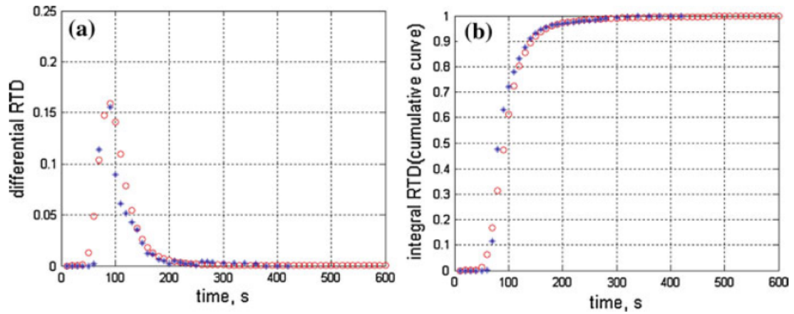
Fig. 6 RTD at 40 rpm and 140°C. a Differential curve, b cumulative curve
