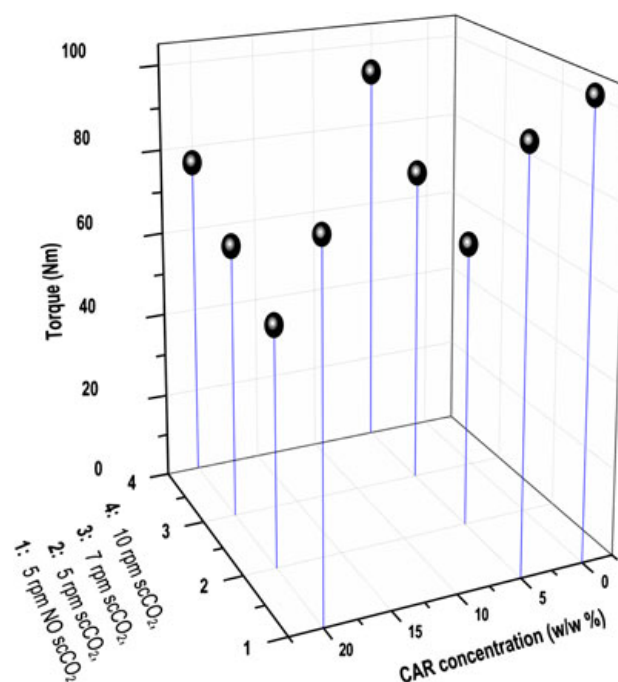
Figure 4. The measured torque during the extrusion in the function of carvedilol (CAR) concentration, screw rotation speed, and CO 2 addition.
