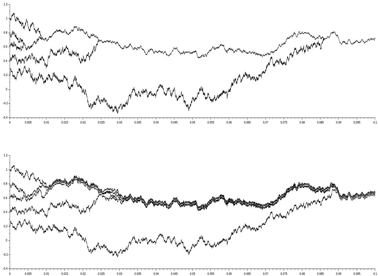
Figure 1: Two simulations, based on the same underlying Brownian sheet, for the limit process (\mu_t)_{t \in [0, T]} (on top) and for the process (\mu_t^{\sigma, \varepsilon})_{t \in [0, T]} with positive \sigma and \varepsilon (on bottom). The horizontal axis represents time. On the vertical axis, we put the position of the particles (initially, we took five particles on [0, 1] ).
