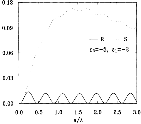
FIG. 9. Reflection and scattering coefficients for a system consisting of a metallic inclusion ( \epsilon_2 = -5 ) in a metal host ( \epsilon_1 = -2 ), when the inclusion touches the interface ( h = 0 ). The other parameters are b = \lambda/20 and \Delta x = \lambda/40 .
