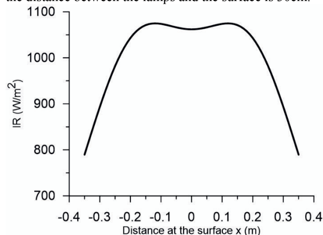
Figure 4: Direct infrared radiation IR at the soil surface calculated for the two infrared lamps
