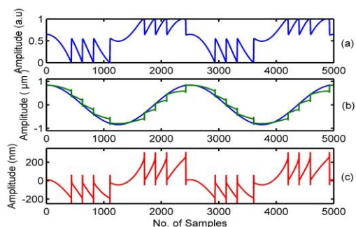
Fig. 11: Displacement reconstruction using CSU for C = 5.0 , \alpha = 5 and \lambda = 785\text{nm} ; (a) SM signal ; (b) Reconstructed D(t) using CSU (green) and Reference Displacement (blue); (c) Error in reconstructed displacement.
