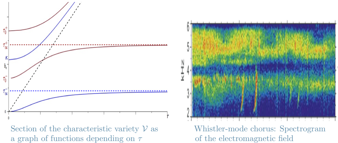
FIGURE 7. Correspondance between cold resonances and spectrograms [8].
