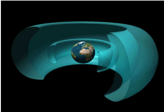
Magnetospheres (cold plasmas [6])
