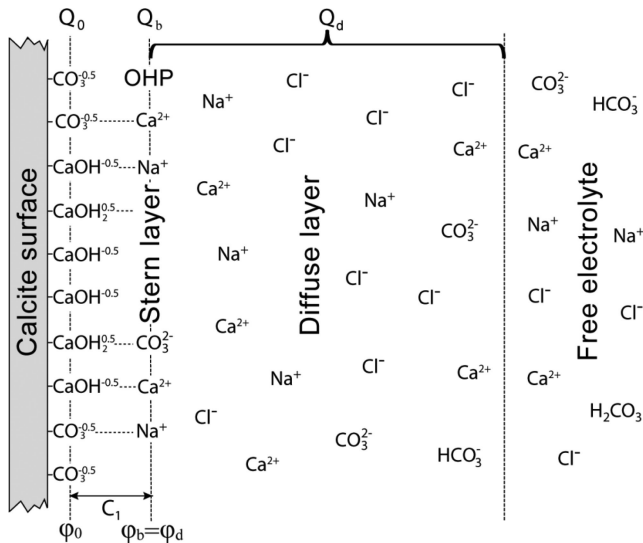
Figure 4. The basic Stern model used by Heberling et al. (2014) to describe the calcite/water interface (calcite (1 0 4) surface) when calcite is in contact with a NaCl and CaCl 2 aqueous solution at equilibrium with a pCO 2 . The parameters \varphi and Q are the electrical potential and surface charge density, respectively, at the 0-plane, b -plane (Stern plane) and d -plane (onset of the diffuse layer). According to the basic Stern model, the onset of the diffuse layer coincides with the Stern plane, that is \varphi_b = \varphi_d . OHP is the Outer Helmholtz plane. The parameter C_1 is the capacitance to model the electrical potential behaviour between the 0-plane and b -plane.
