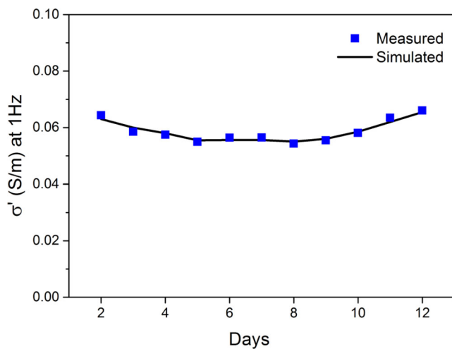
Figure 9. In-phase conductivity of the calcite precipitation experiment of Wu et al. (2010). In-phase conductivities inferred from the complex conductivity model are represented by the line and the symbols represent the real conductivity measurements of Wu et al. (2010).
