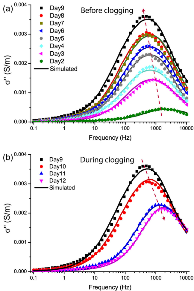
Figure 6. Imaginary conductivity spectra of calcite precipitation on glass beads as a function of time in days (after the beginning of the experiment) before the pore clogging by the calcite precipitates (a) and during the pore clogging by the calcite precipitates (b). Imaginary conductivities inferred from the complex conductivity model are represented by the lines and the symbols represent the imaginary conductivity measurements of Wu et al. (2010).
