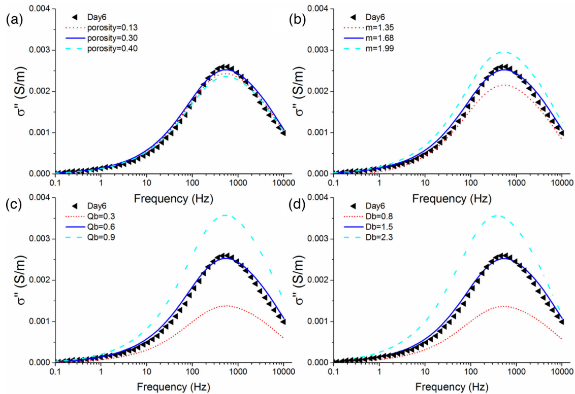
Figure 5. Effects of porosity of glass beads pack \phi (a), cementation exponent m (b), surface charge density of the Stern layer Q_b (in C\ m^{-2} ) (c) and diffusion coefficient D_b (in 10^{-10}\ m^2\ s^{-1} ) (d) on the modelled imaginary conductivity. The computations of the complex conductivity model are represented by the lines and the symbols represent the imaginary conductivity measurements of Wu et al. (2010).
