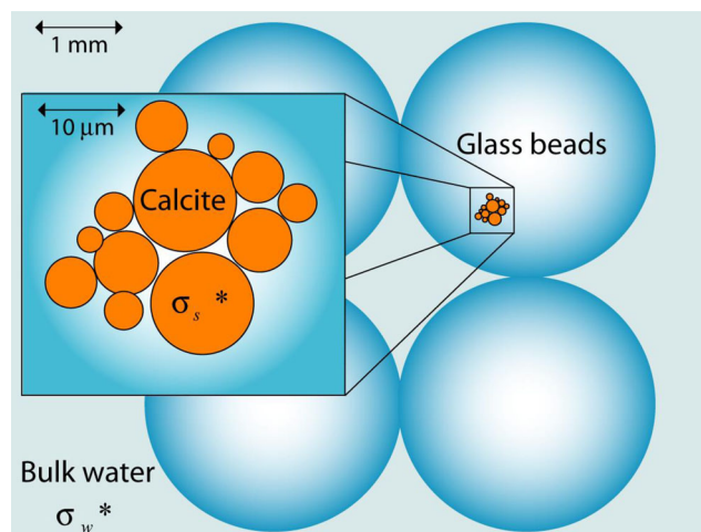
Figure 1. Sketch of our complex conductivity model of the porous medium. Parameters \sigma_w^* and \sigma_s^* are the complex bulk water and surface conductivity of solid, respectively. Calcite particles are mostly rhombohedral, but considering them spherical is a good first approximation.
