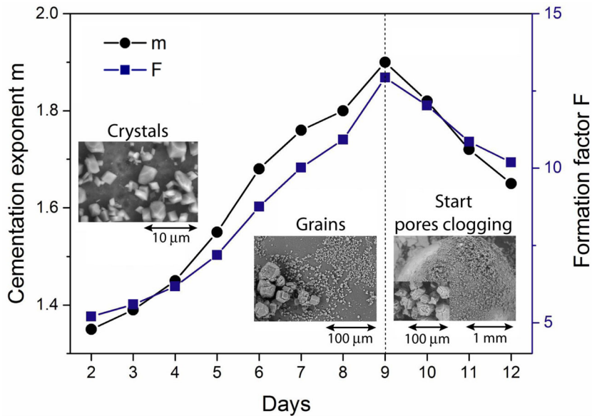
Figure 8. Computed particles cementation exponent ( m ) and formation factor F changes during the calcite precipitation experiment of Wu et al. (2010). The cementation exponent and formation factor of the glass beads pack where calcite precipitation occurs have a different trend of changes before and after the starting of the pore clogging (day 9).
