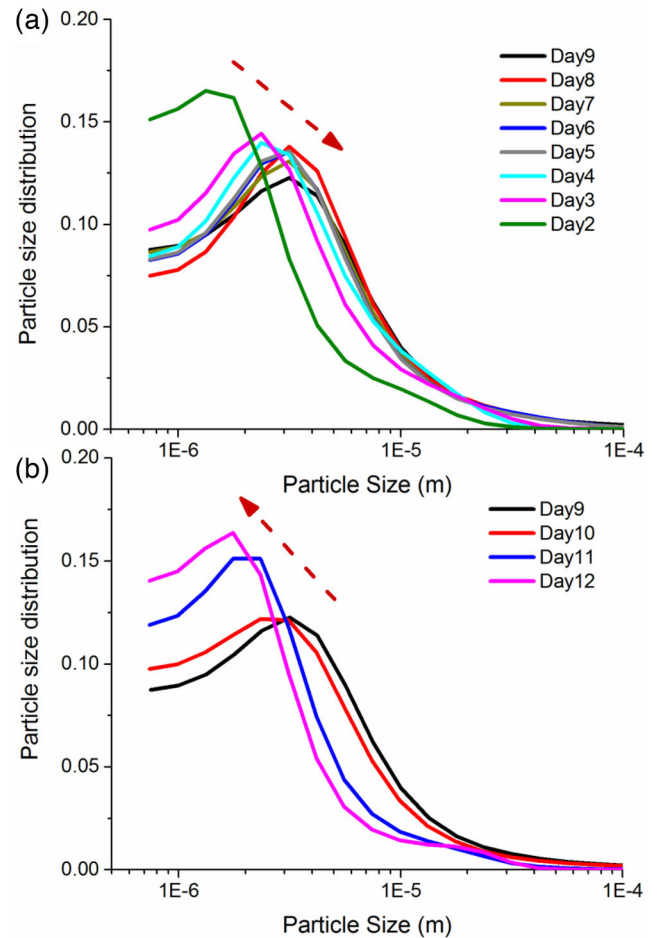
Figure 7. Evolution of the computed particle size distribution of calcite particles during calcite precipitation experiment obtained from the relaxation time distribution (RTD) code (Florsch et al. 2014).
