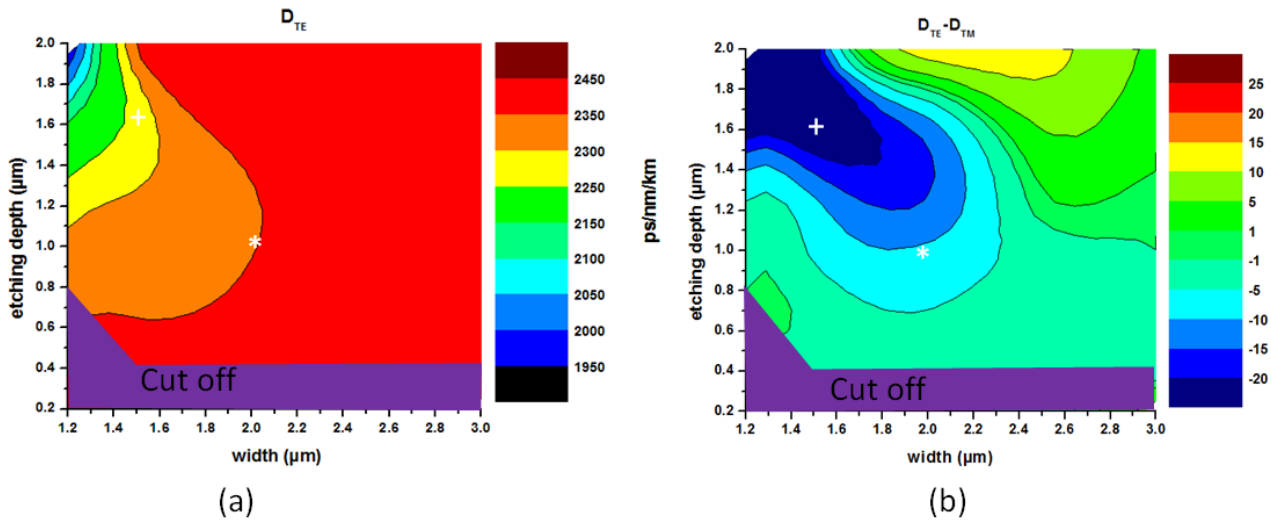
Figure 4. Influence of geometrical parameters on: TE dispersion coefficient (a), dispersion coefficient birefringence D_{TE} - D_{TM} (b), *configuration 1 waveguide position, +-configuration 2 waveguide position
