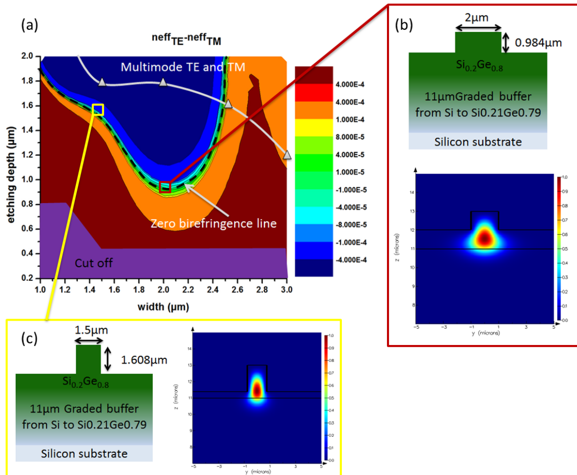
Figure 2. Waveguide effective index birefringence optimization: (a) \Delta n_{\text{eff}} = n_{\text{eff}_{\text{TE}}} - n_{\text{eff}_{\text{TM}}} maps, (b) cross section and optical mode of optimized waveguide: configuration 1 (c) cross section and optical mode of optimized waveguide: configuration 2
