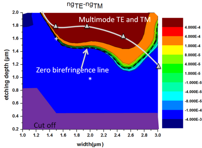
Figure 3. Influence of geometrical parameters on group index birefringence: \Delta ng = ng_{TE} - ng_{TM} maps, *-configuration 1 waveguide position, +-configuration 2 waveguide position
