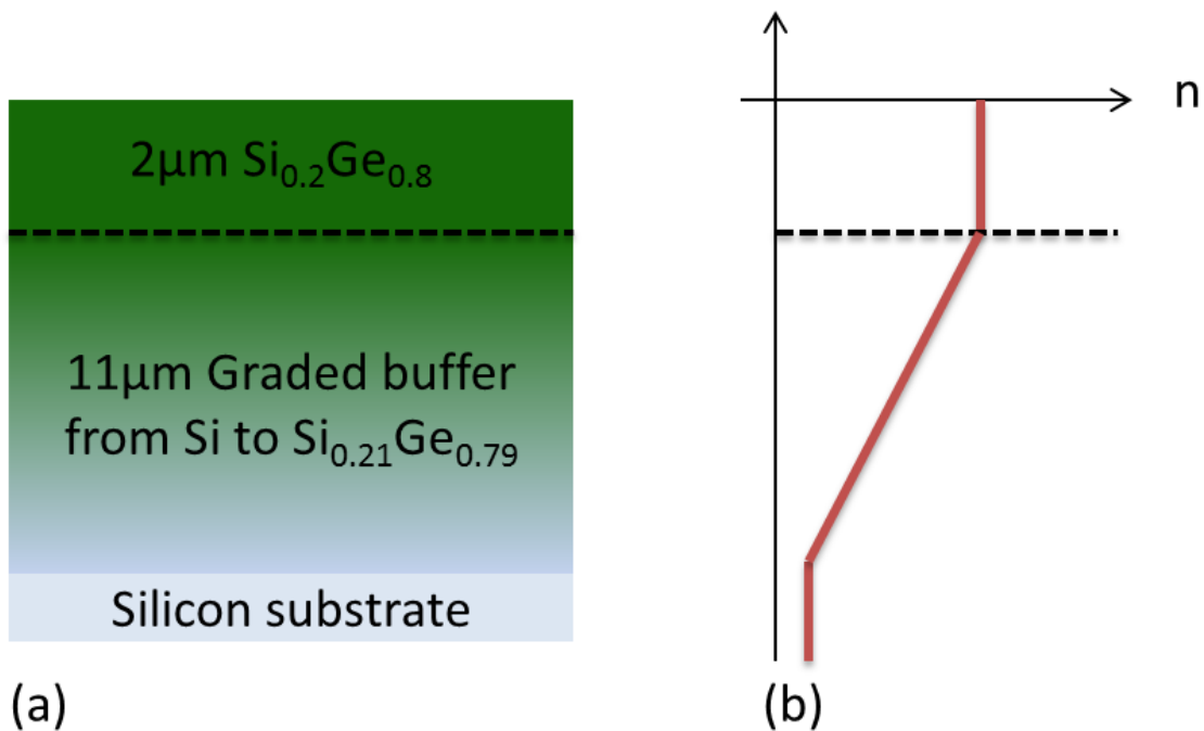
Figure 1. Ge-rich SiGe material platform: (a) epilayer grown by LEPECVD on standard silicon substrate, (b) refractive index evolution along the growth direction
