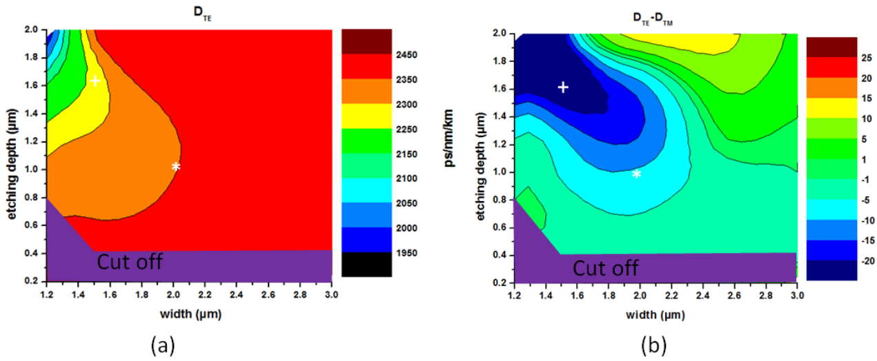
Figure 4. Influence of geometrical parameters on: TE dispersion coefficient (a), dispersion coefficient birefringence D_{TE}-D_{TM} (b), *configuration 1 waveguide position, +-configuration 2 waveguide position
