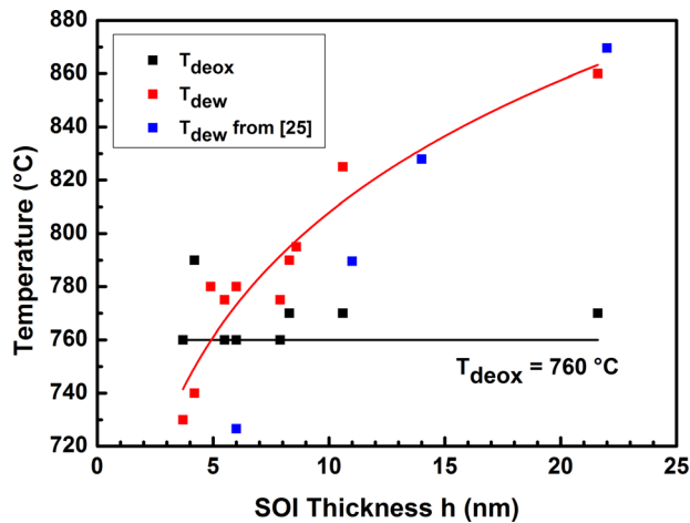
FIG. 1. Temperature at which the initial deoxidation (black) and dewetting (red) are observed as a function of the Si film thickness. Dewetting velocities are in the range of 1 to 8 nm/s. The data point at 21.6 nm was obtained using a SOI sample of 22 nm on top of a 150 nm SiO 2 BOX. The blue data points are obtained from 25 with a dewetting velocity of 3 nm/s.
