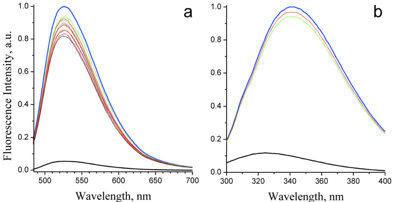
Fig 1. Noncovalent binding of free FMN to apoNqrC' studied by the flavin and the protein fluorescence shown on the left and right panels, respectively. (a) Fluorescence of 0.35 μM free FMN (thick blue line) and 0.35 μM holoNqrC' (thick black line). The thin lines represent titration of fluorescence of free FMN (0.35 μM) by increasing amounts of apoNqrC' (apoNqrC' concentrations varied from 0.08 to 45 μM). (b) Tryptophan fluorescence of 0.32 μM apoNqrC' (thick blue line) and 0.32 μM holoNqrC' (thick black line). The red and green thin lines represent fluorescence of 0.32 μM apoNqrC' in the presence of 0.32 and 0.64 μM of free FMN, respectively.
