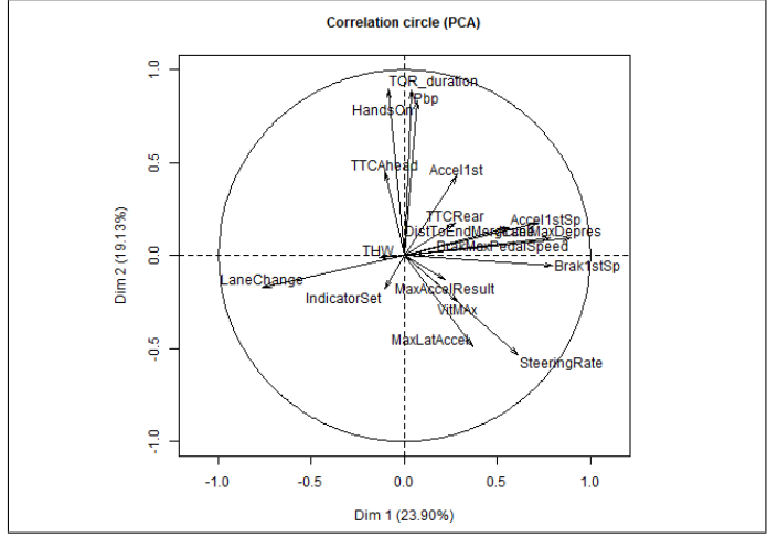
Fig. 1: Vehicle variables
