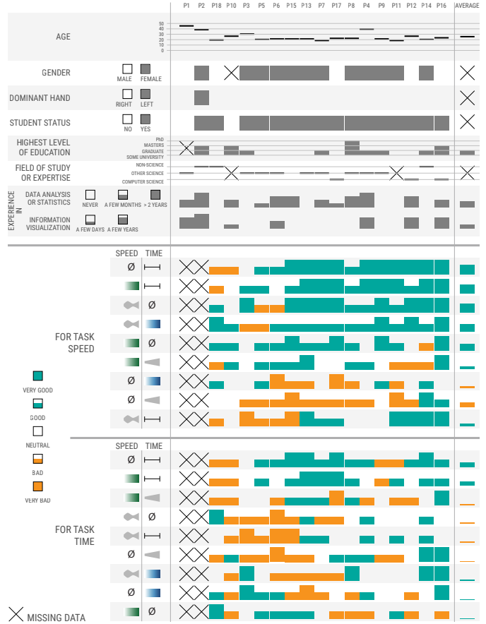
Fig. 11. Participant demographics and 1–5 Likert scale answers for each encoding and task. Participants were reordered using Bertifier [59] according to the similarity of the scores they gave to each encoding. Encodings were vertically reordered independently for SPEED and for TIME according to the similarity of the scores they received.
