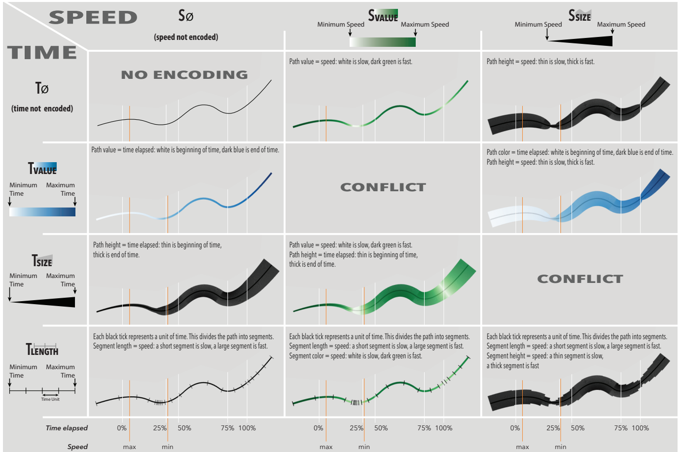
Fig. 9. Time and speed encodings on 2D paths. Speed can be: not encoded ( S_{\emptyset} ) or encoded using value ( S_{VALUE} ) or size ( S_{SIZE} ). Time can be: not encoded ( T_{\emptyset} ) or encoded using value ( T_{VALUE} ), size ( T_{SIZE} ), or length ( T_{LENGTH} ). We tested all nine encodings that convey at least one of speed and time.
