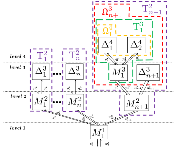
Fig. 1: Uncertain linear large scale system T_1^1 with hierarchical structure of four levels
