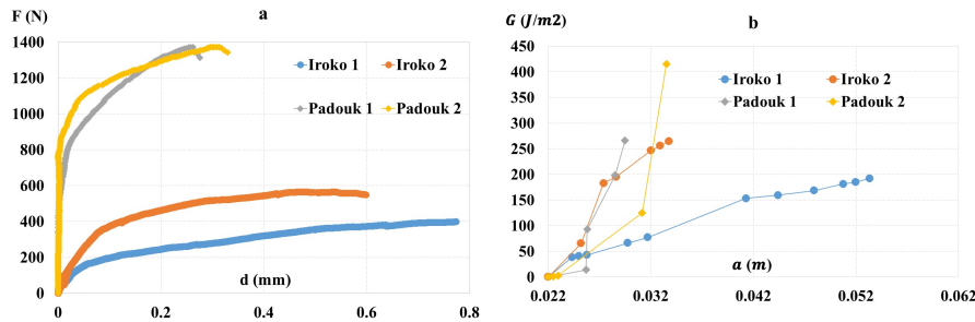
Figure 2. Force-displacement curves (a) and critical energy release rate- crack length curves (b). Padouk 1 and Iroko 1 specimens of thickness 15mm and Padouk 2 and Iroko 2 specimens of thickness 20mm.
