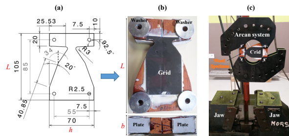
Figure 1. dimensions of specimen (a); side view of the notched specimen equipped with a grid (b), experimental device (c)
