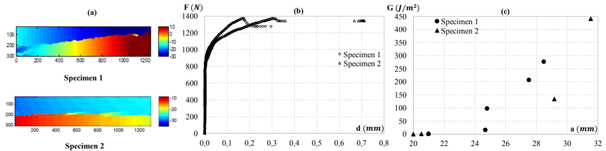
Figure 2: displacement maps (a), force-displacement curves (b), Critical energy release rate (c)
