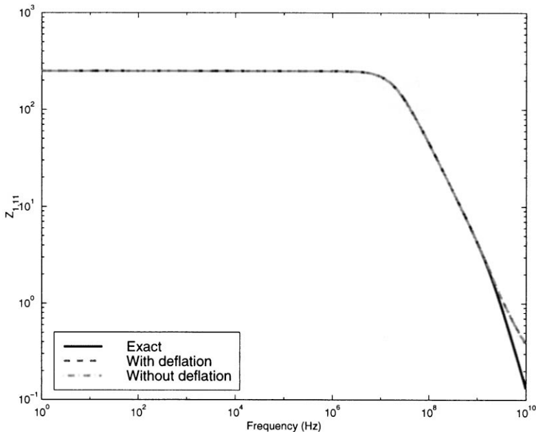
Fig. 4. Impedance H_{1,11} .
