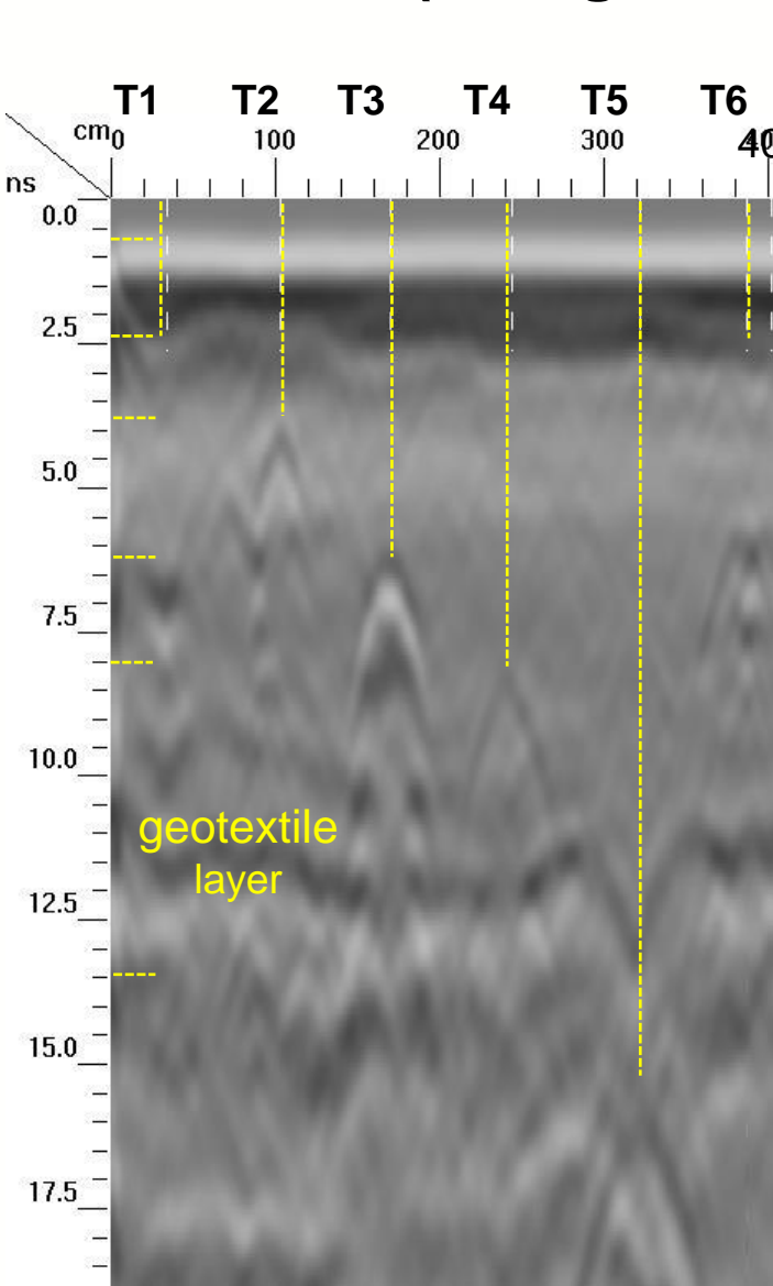
800 MHz (with gain)
