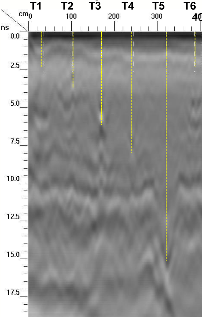
800 MHz (time zero correction and migration ε²=12.75)
