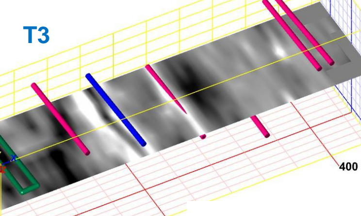
(c) depth 23.6 cm
