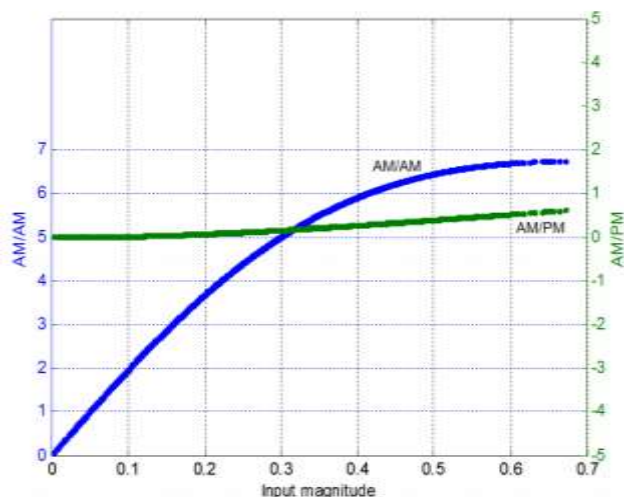
Fig. 2. AM/AM and AM/PM characteristics for a Typical PA
