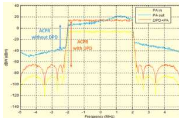
Fig. 4. Example of Adjacent channel power ratio (ACPR) improvement with DPD
