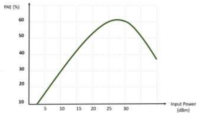
Fig. 3. PA Power Added Efficiency (PAE)
