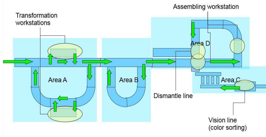
Figure 3: TRACILOGIS flowchart
