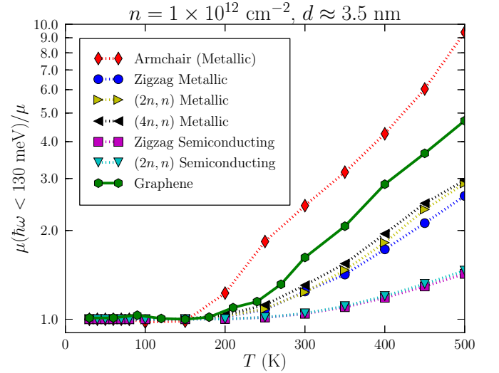
FIG. 4. (Color online) Ratio between the mobility calculated by considering phonons with energy below 130 meV and the mobility calculated with all phonons vs temperature. d \approx 3.5\text{ nm} , n = 10^{12}\text{ cm}^{-2} .
