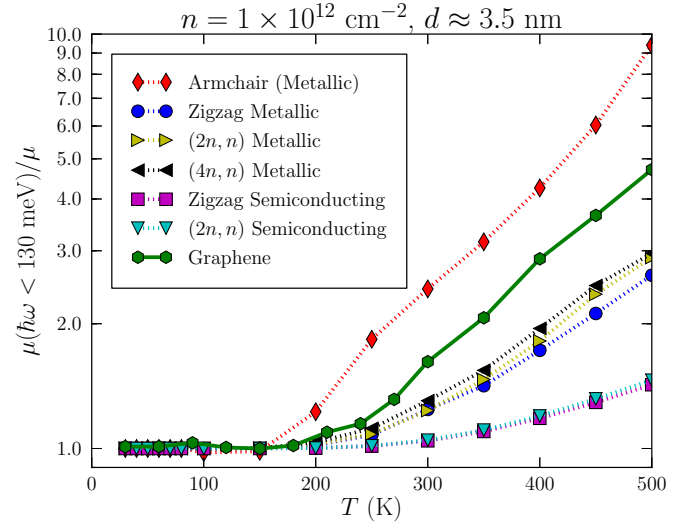
FIG. 4. (Color online) Ratio between the mobility calculated by considering phonons with energy below 130 meV and the mobility calculated with all phonons vs temperature. d \approx 3.5 nm, n = 10^{12} cm ^{-2} .
