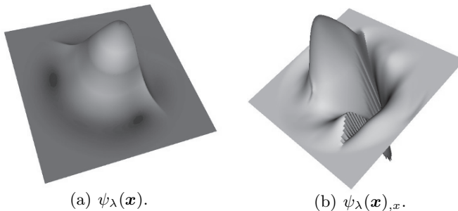
Figure 2. Enriched shape function and its derivative evaluated for a node close to a circular interface
