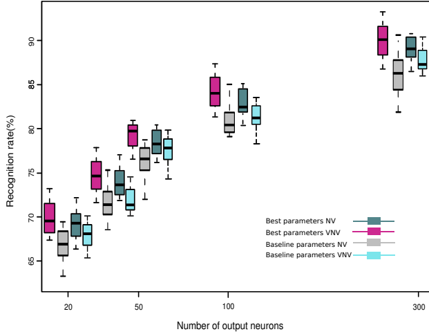
Fig. 14. Using the best parameters significantly improves the recognition rate.
