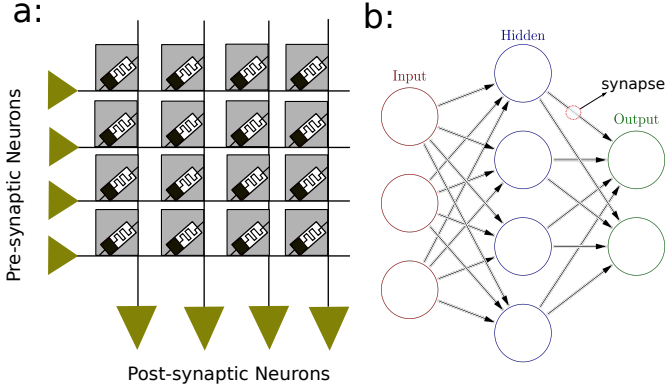
Fig. 1. Crossbar arrays allow to build SNNs. a) The memristive synapse connects the spiking neurons in configurable crossbar array suitable for STDP unsupervised learning, the presynaptic neurons are considered as inputs and postsynaptic neurons as outputs. b) Two crossbar arrays can interconnect the neurons of a three-layer feed-forward SNN.
