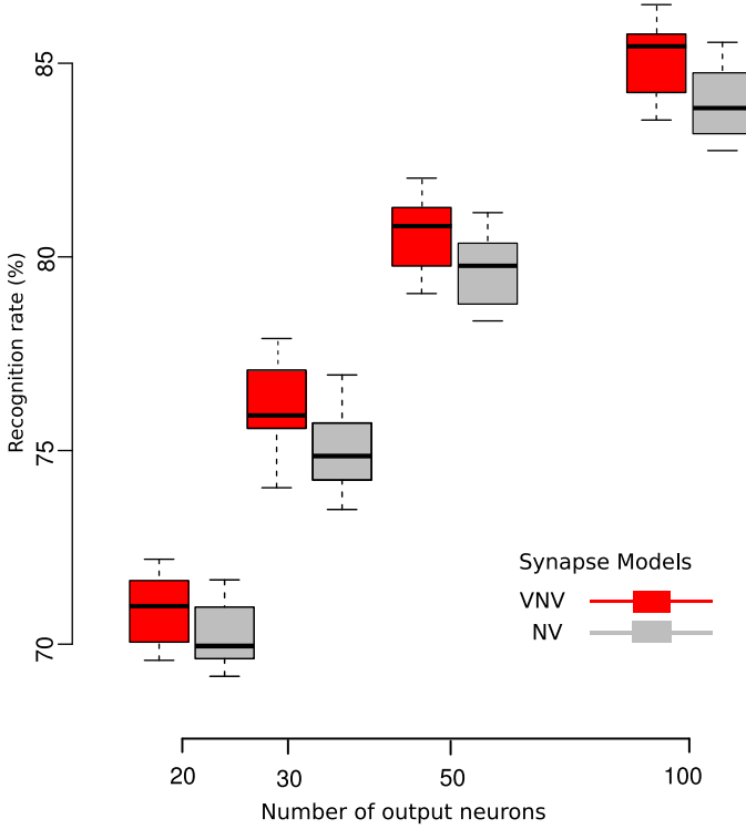
Fig. 4. Recognition rate as a function of number of output neurons. In the box plot (with the default parameters of the R boxplot function) for each number of neurons, we compare the recognition rate of the two synapse models.
