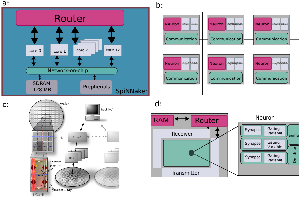
Fig. 2. Large scale spiking neural network systems, a) Principal architectural parts of a SpiNNaker processing node, b) In TrueNorth, conceptual blueprint of an architecture like the brain, tightly integrates memory, computation, and communication in distributed modules that operate in parallel and communicate via an event-driven. c) Schematic of HICANN board in BrainScales project, d) In Neurogrid, the chip comprises a 256 \times 256 array of neuron elements, an asynchronous digital transmitter for sending the events generated by the neurons, a receiver block for accepting events from other sources, a router block for communicating packets among chips, and a memory blocks for supporting different network configurations.
