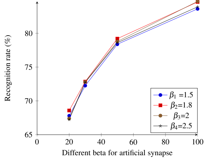
Fig. 13. comparing network performance using various number of neurons with different fitting parameter ( \beta ) for synapse model.
