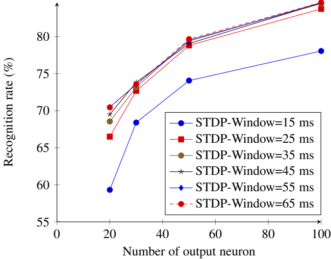
Fig. 9. Average recognition rate of the network using different number of neuron and six different STDP window durations.
