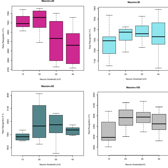
Fig. 10. Comparison of the recognition rate for various neuron thresholds.
