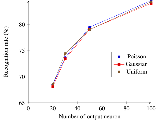
Fig. 7. Average recognition rate of the network using different input spike train distributions.
