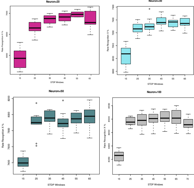
Fig. 8. The comparison of different STDP window durations.
