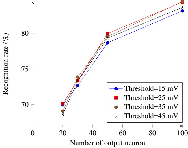
Fig. 11. Average recognition rate for various neuron thresholds.
