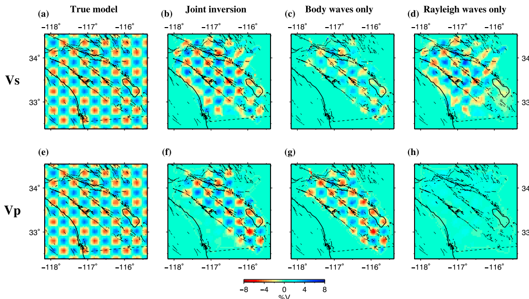
Figure 6. Comparison of recovered checkerboard models using body waves or Rayleigh waves at 7 km depth. (a) Input V_s model, (b) recovered V_s model from joint inversion of body and Rayleigh waves, (c) recovered V_s model using body waves only, and (d) recovered V_s model using Rayleigh waves only; (e) input V_p model, (f) recovered V_p model from joint inversion, (g) recovered V_p model using body waves only, and (h) recovered V_p model using Rayleigh waves only.
