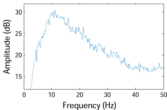
Figure 3. Averaged power-spectral density obtained for sensor R2307 for one day of recording (Julian Day 150).
