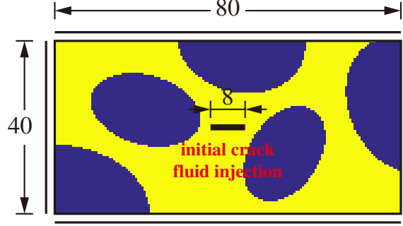
Fig. 10. A heterogeneous medium with ellipsoidal inclusions subjected to a constant fluid injection on an initial crack. All edges are mechanically restrained and are assumed to be permeable.
