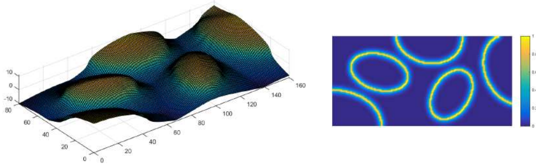
Fig. 12. Interface phase field determination: (a) level-set function \psi(\mathbf{x}) constructed as a signed distance function of the heterogeneous medium in Fig. 10, (b) the correspondingly determined interface phase field \beta(\mathbf{x}) .
