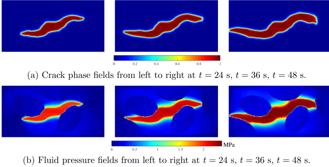
Fig. 11. Evolution of the crack phase and fluid pressure during the hydraulic fracturing of the heterogeneous medium without considering the cohesive interfacial effect.
