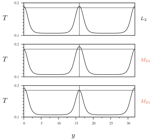
Fig. 5. Comparison of the L_2 solution (top panel) with the M_{21} solution (lower panels) at x = 0 . The solutions in the lower panels are related by translation through L_j/2 . The thin horizontal line connects the peaks with the smaller amplitude and is drawn to emphasize the height differences arising from spatial modulation of the L_2 state in the top panel. The Damköhler numbers are ( L_2 ) 1229.7331, ( M_{21} ) 1245.8670, and ( M_{21} ) 1244.0886.
