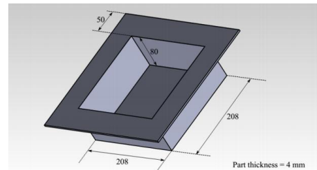
Fig. 11: Part model
