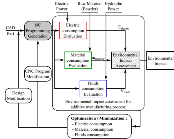
Fig. 10: Global methodology to evaluate the environmental impact of CAD part
