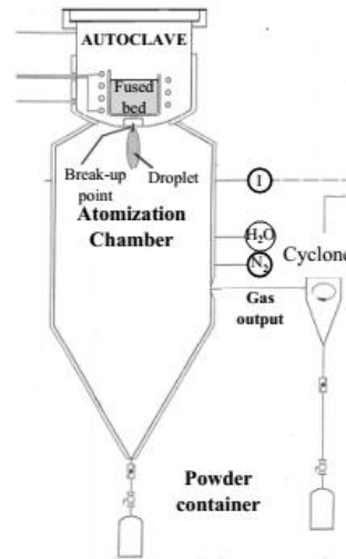
Fig. 7: Atomization process [13]
