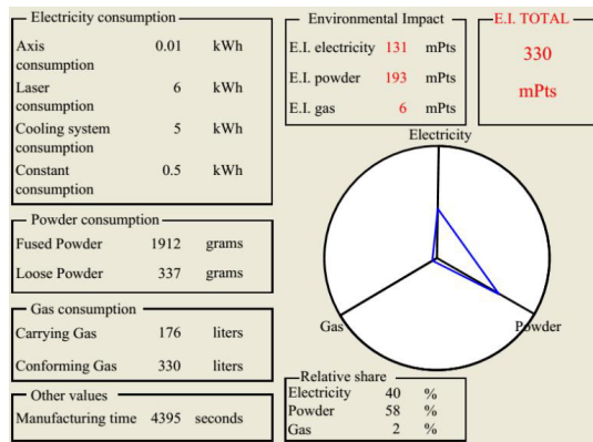
Fig. 12: MacroCLAD results
