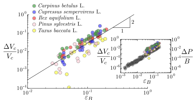
Fig. 55. Normalized expelled volume of water as function of the bending deformation (the maximal deformation at the center of the branch in a four-point bending setup) on five tree species [computed from the raw data of Lopez et al., 2014 (23)]. The best quadratic fit of the data gives \Delta V_c / V_c = (2.90 \pm 0.25) \times \varepsilon_B^2 ( R^2 = 0.68 ).
