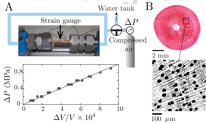
Fig. S4. Measurement of the channel bulk modulus in poplar branches ( P. alba × tremula L.). (A) Experimental setup used to determine the macroscopic bulk modulus B_{\text{macro}} from the relationship between the pressure increments \Delta P and the relative change of the branch's volume \Delta V/V (see plot, here B_{\text{macro}} = 1 \pm 0.02 GPa). (B) Cytological cross-section for measurement of the channel's fraction \psi (in black) and estimation of B via the relation B = \psi B_{\text{macro}} .
