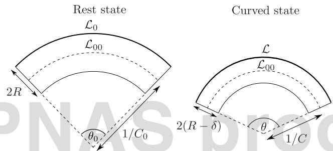
Fig. S3. Illustration of flattening of an initially curved beam induced by bending.
