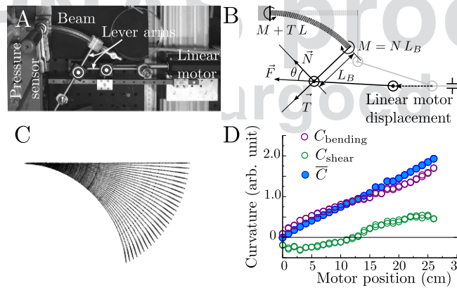
Fig. S1. (A) Top view of the bending setup, including a linear motor, lever arms, and rotating bearings. (B) Force balance on the bent beam. Once the displacement is imposed, the beam is subject to a force F which creates a bending moment M = NL_B , a compression force N , and a tangential force T . (C) Beam's profiles extracted by image analysis from top views during a sequence of motor displacements. Each profile is fitted by a law such that C(x) = C_{\text{bending}} + C_{\text{shear}}(1 - (x/L)) , where C_{\text{bending}} and C_{\text{shear}} are fitting parameters and x is the coordinate along the beam. (D) Curvatures measured from the beam profiles as function of the displacement of the motor where \bar{C} = C_{\text{bending}} + (C_{\text{shear}}/2) .
