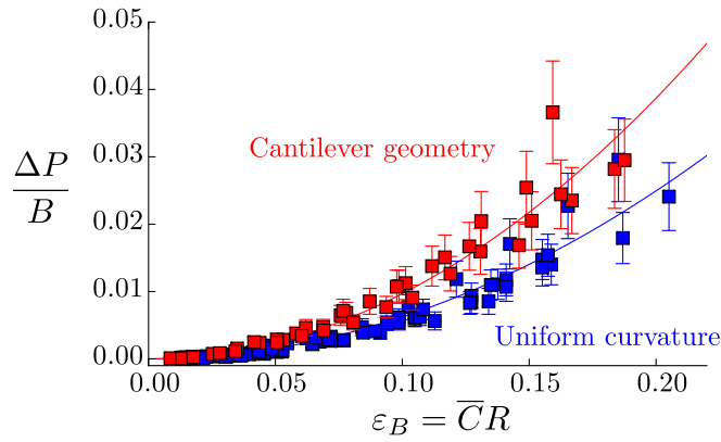
Fig. S2. Pressure response to bending normalized by the elastic bulk modulus of the biomimetic branches as function of the bending deformation \varepsilon_B = \overline{C}R for a uniform curvature (blue symbols, quadratic fit y = 0.62x^2 ) and a linear variation of curvature (red symbols, quadratic fit y = 0.97x^2 ) (synthetic beams). Insets give the measured distribution of curvature along the beams normalized by the beam's length L in both cases.
