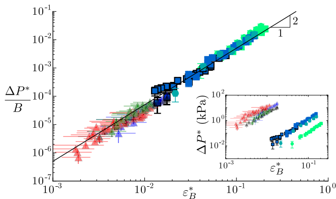
Fig. 5. Comparison between biomimetic (squares; same symbols as in Fig. 3) and natural tree branches (triangles; same symbols as in Fig. 4). The overpressure \Delta P^* normalized by the elastic bulk modulus B of each branch shows a common behavior with the amplitude of the bending strain \varepsilon_B^* . The solid line represents the best quadratic fit of all data in log-log scale: \Delta P^*/B = (0.50 \pm 0.01) \times \varepsilon_B^{*2} ( R^2 = 0.98 ). (Inset) Overpressure vs. bending strain for all data.
