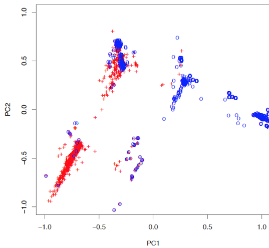
Figure 4: Visualizing samples in 2-dimensions: Love (red crosses) vs. Pleasure (blue circles)
