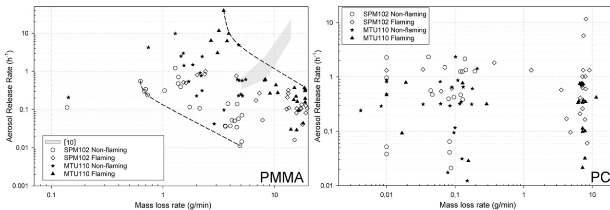
Fig. 9. Al 2 O 3 release rate (% per hour) as a function of mass loss rate for PMMA (left) and PC (right).
