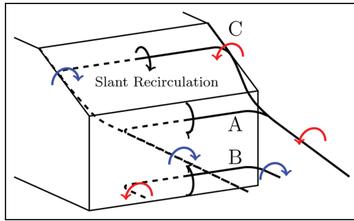
Figure 10. Vortex structure schematic in the wake of the Ahmed body, with lines indicating the location of the vortex cores. The structure is dashed for y/W < 0 and solid for y/W > 0 . Spanwise rotation is indicated by black arrows and streamwise rotation is indicated by red or blue arrows for positive or negative rotation, respectively.
