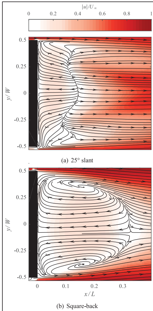
Figure 7. (a) Flow in the xy plane at z/H = 0.369 with velocity streamlines overlaid onto filled contours of total velocity. (b) Flow behind the square-back Ahmed geometry at the mid-height plane clearly showing the vertical legs of the toroidal vortex. Streamlines are used to indicate the local flow direction only.
