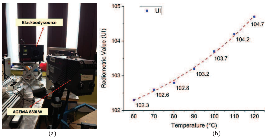
FIGURE 2. Test set-up for calibration of IR camera with the optical filter at 7.6\ \mu\text{m} (a) and the calibration curve obtained for the reference temperatures between 60 and 120\ ^\circ\text{C} (b).
