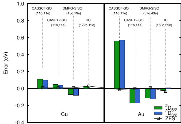
FIG. 2. Errors (eV) in the individual 2 D 5/2 and 2 D 3/2 states of the coinage atoms (bars), as well as of the ZFS between the two (black line) of different methods previously reported and of SHCI calculations from this work. Although the ZFS is well reproduced by all methods, SHCI performs well in its description of the individual states.
