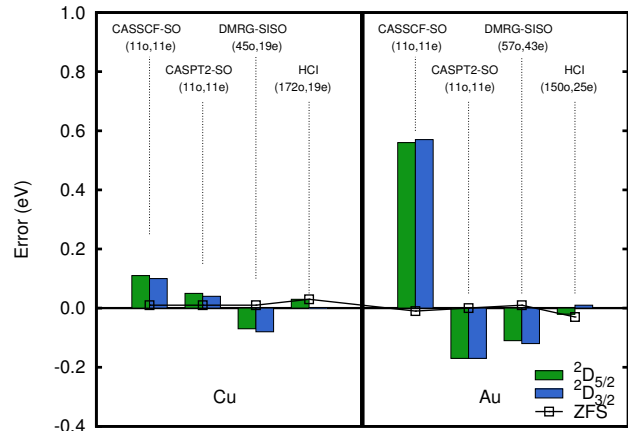
FIG. 2. Errors (eV) in the individual ^2D_{5/2} and ^2D_{3/2} states of the coinage atoms (bars), as well as of the ZFS between the two (black line) of different methods previously reported and of SHCI calculations from this work. Although the ZFS is well reproduced by all methods, SHCI performs well in its description of the individual states.
