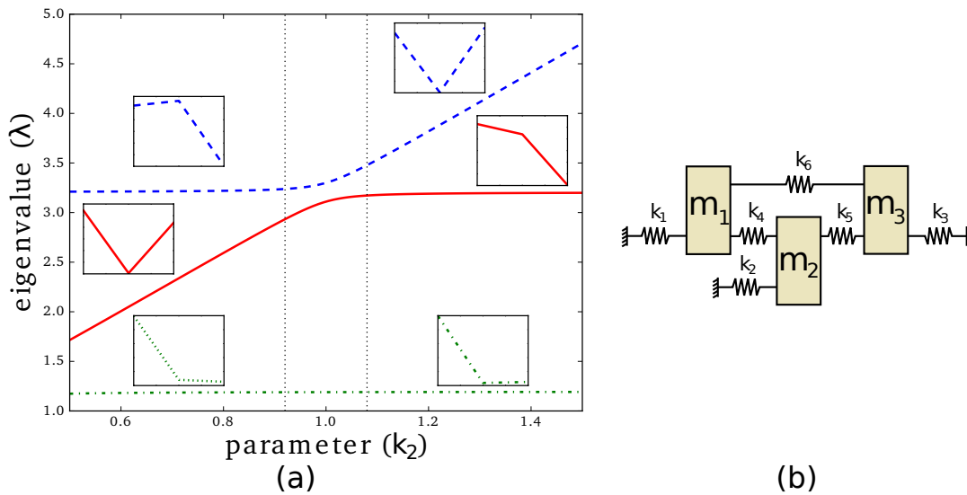
Figure 1: Eigenvalue loci with the corresponding eigenvector (a) of a 3 DoF system (b)
