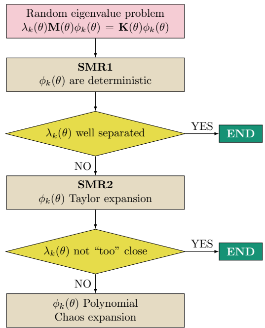
Figure 3: SMR approach for eigenvalue problem resolution
