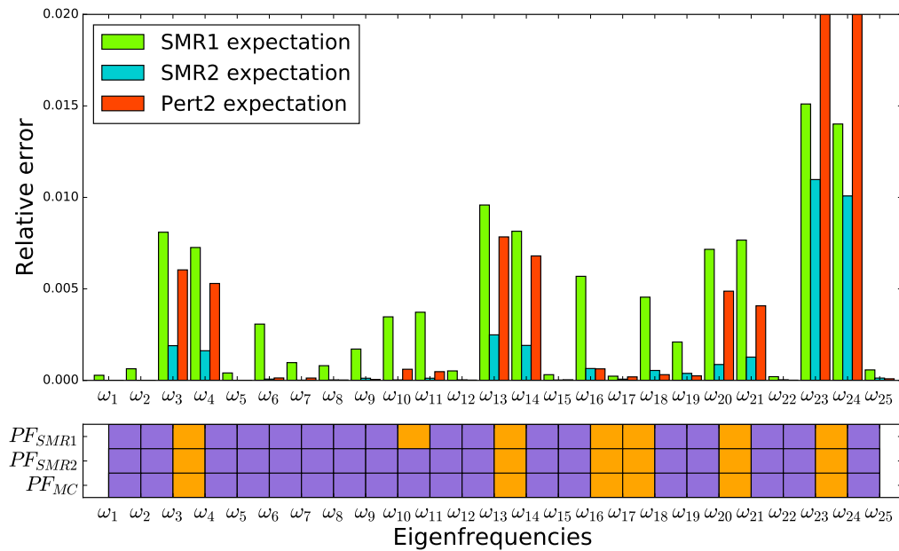
Figure 16: Relative error of the estimation of the expectation for the first 25 random eigenfrequencies
