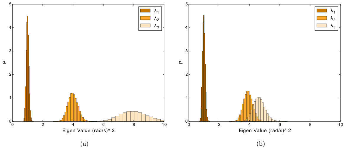
Figure 5: Superposition of all eigenvalue marginal density functions. (a) All eigenvalues are well separated. (b) Two eigenvalues are close
