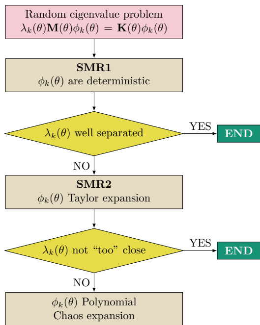
Figure 3: SMR approach for eigenvalue problem resolution
