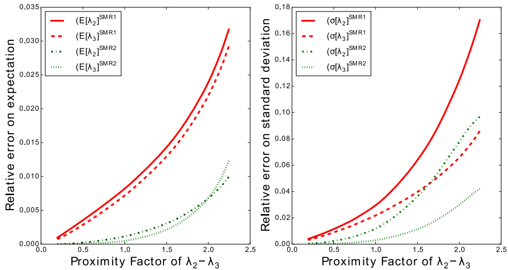
Figure 8: Error on the estimation of the first moments when PF increase
