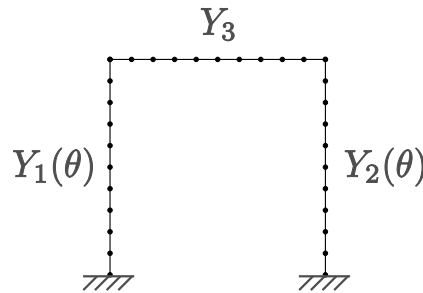
Figure 11: Definition of the three beams frame
