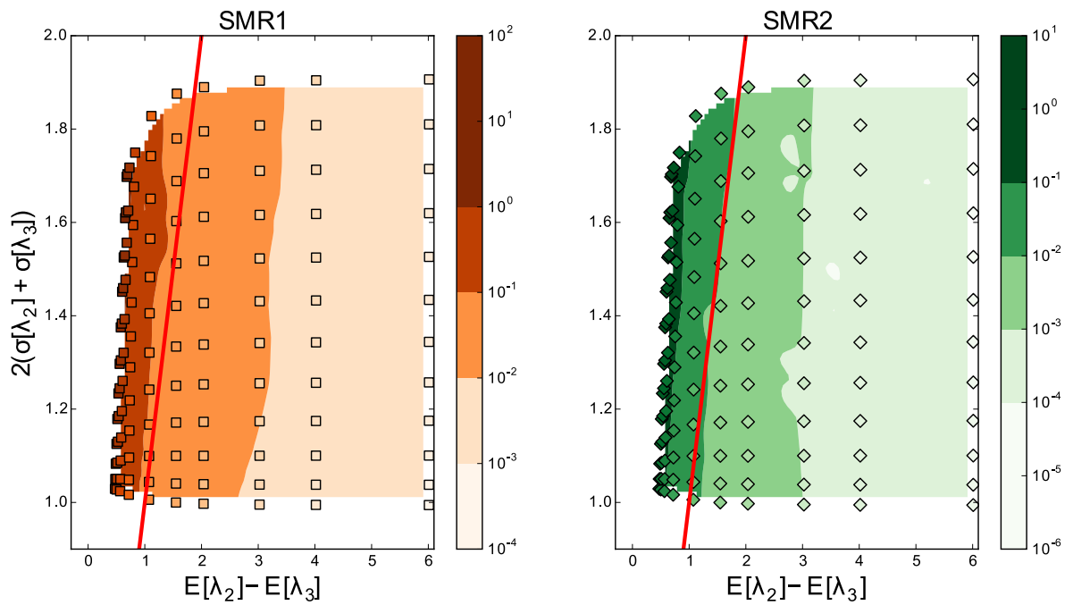
Figure 10: Relative error of the Proximity Factor respectively computed with SMR1 and SMR2
