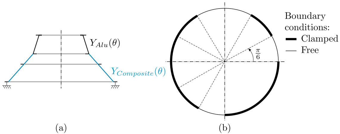
Figure 20: Definition of the Ariane 5 Payload Adapter PAS 1666MVS. (a) Section of the PAS 1666MVS. (b) Definition of the clamped boundary conditions of the lower cone.
