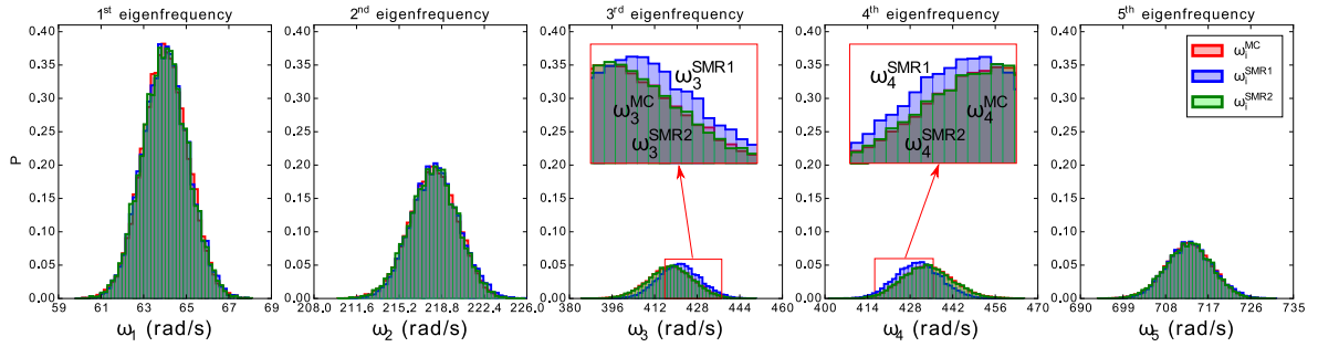
Figure 13: Marginal density functions of the first five eigenfrequencies estimated with SMR1 and SMR2
