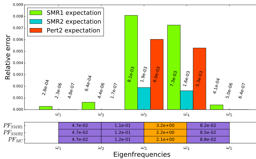
Figure 14: Relative error of the expectation estimated with SMR1, SMR2 and the second order perturbation method
