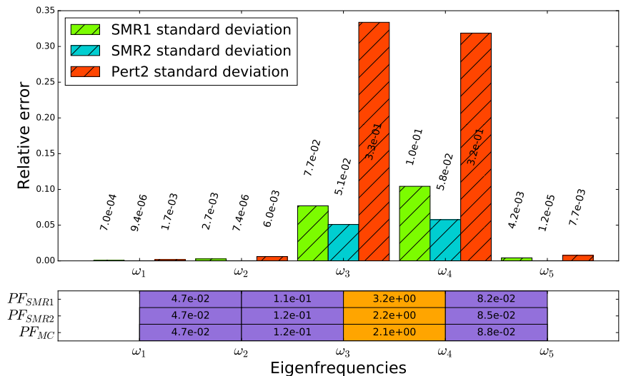
Figure 15: Relative error of the standard deviation estimated with SMR1, SMR2 and the second order perturbation method
