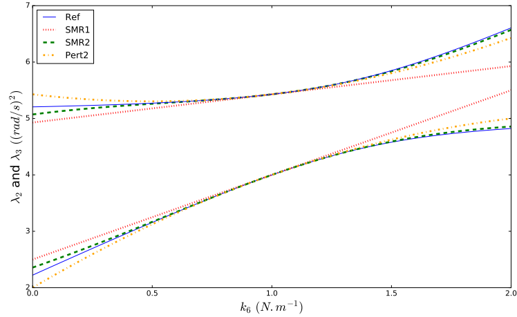
Figure 7: Response surface of the second and third eigenvalues computed with the exact resolution ( Ref ), SMR1, SMR2 and second order perturbation method
