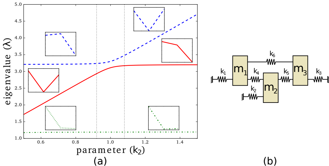
Figure 1: Eigenvalue loci with the corresponding eigenvector (a) of a 3 DoF system (b)
