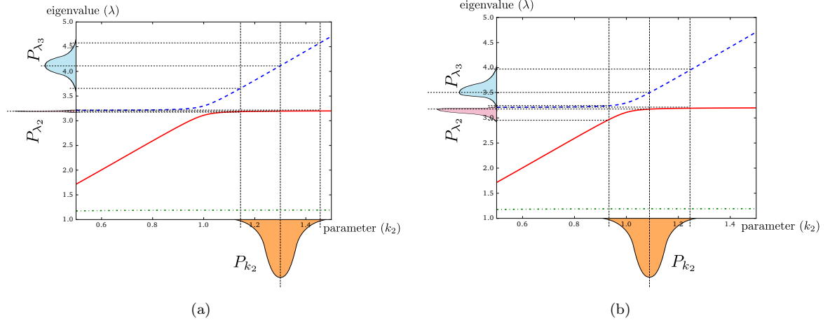
Figure 2: Marginal density functions of the second and third eigenvalues of a three Dof system when the pdf of the input parameter is out of the veering area (a) or cross it (b)
