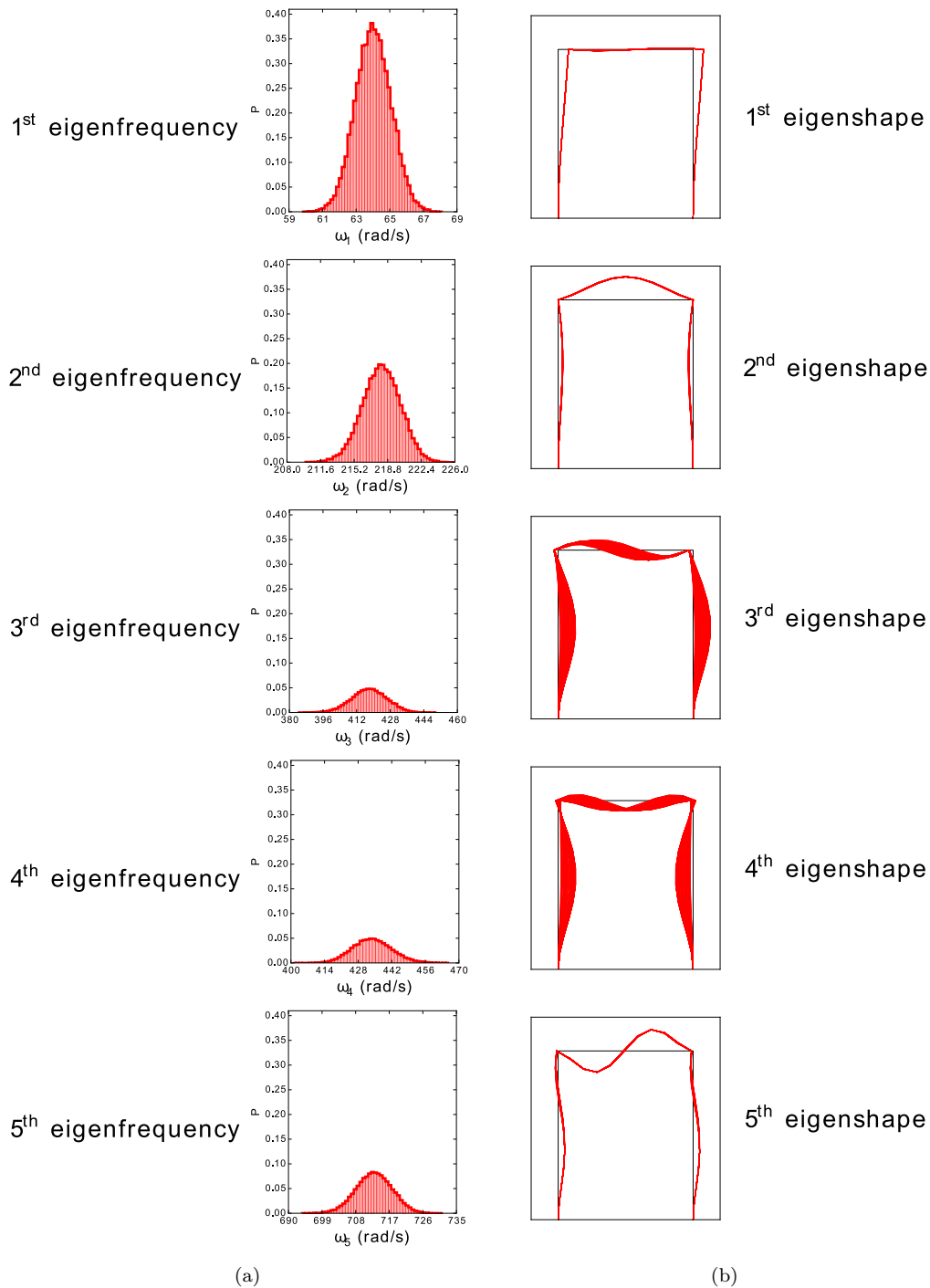
Figure 12: Marginal density of the first 5 random frequencies (a) and the corresponding eigenshapes (b)
