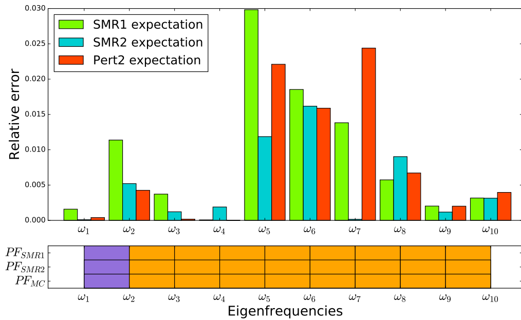
Figure 21: Relative error of the expectation estimation of the PAS first 10 random eigenfrequencies
