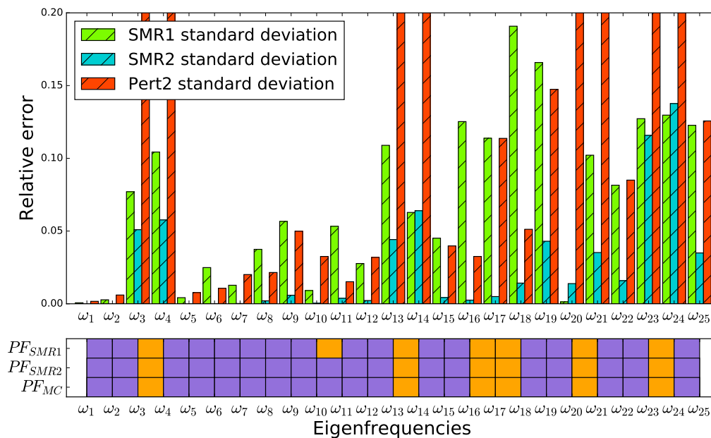
Figure 17: Relative error of the estimation of the standard deviation for the first 25 random eigenfrequencies
