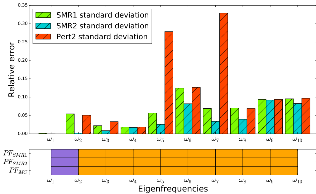
Figure 22: Relative error of the standard deviation estimation of the PAS first 10 random eigenfrequencies
