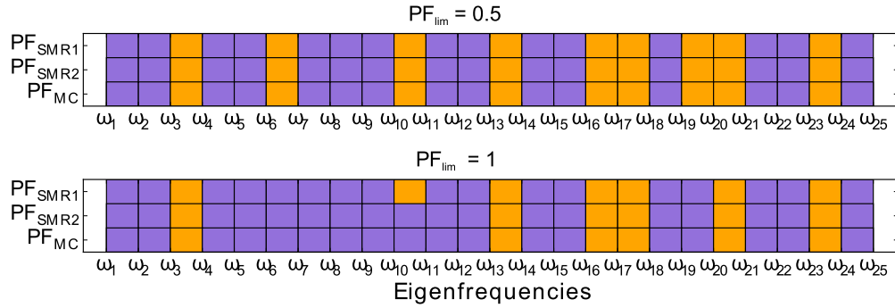
Figure 18: Impact of the limit value of PF on the number of eigenvalues to be refined
